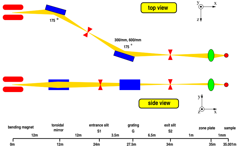
FIGURE 1. Layout of the PoLux beamline.
