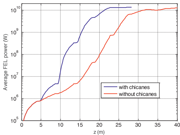
Figure 2.7: FEL power in normal SASE operation (without chicanes) and in optical klystron mode (with chicane) [5].
