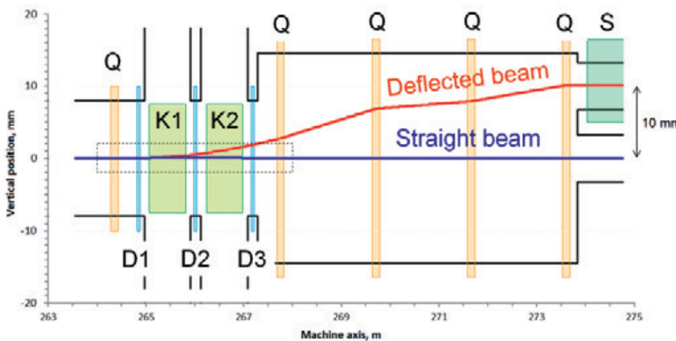
Fig 3.4.6.2. Beam trajectory and field regions in switchyard.
