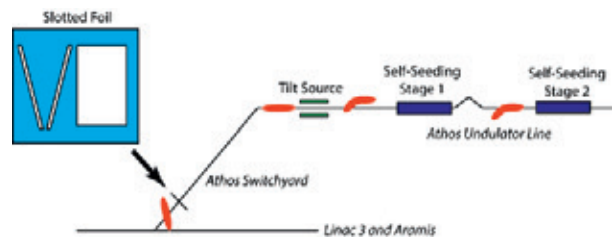
Figure 2.8: Schematic layout for phase-locked pulses in Athos.
