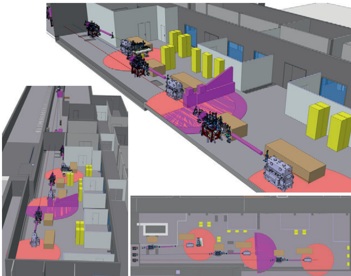
Fig. 4.4.1. Layout of the experimental hall of the Athos beamline, including schematics of the three Athos endstations.
