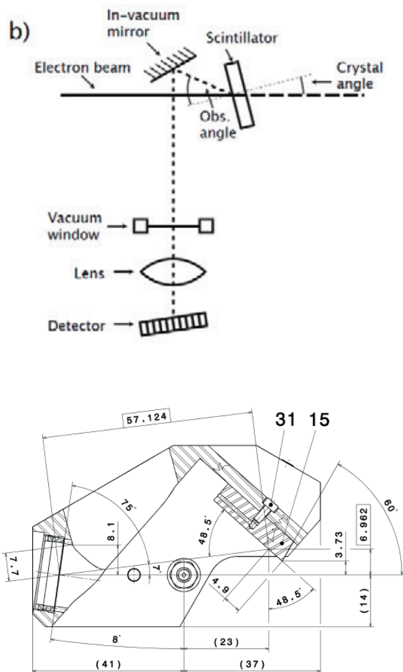
Figure 3.6.2.1: Top: Imaging of the scintillating radiation observing the Snell-Descartes law of refraction as well as the Scheimpflug imaging condition. Bottom: Screen holder for scintillating crystals. Technical drawing, including the scintillator to the left and the in-vacuum mirror to the top right.
