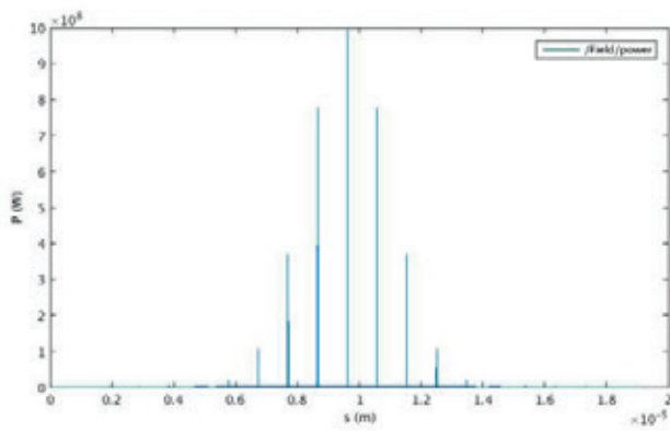
Figure 2.21: Seed signal of HHG pulse to be resonant at 4 nm.
