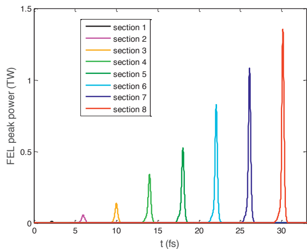
Figure 2.16: FEL radiation profile after each undulator section for L=2m and a tilt of 3 mm in offset.
