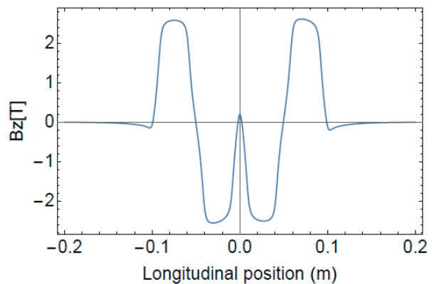
Figure 3.5.4.2: Magnetic field profile along the longitudinal z axis of the chicane. RADIA Simulation done with NdFeB magnets / poles combination.
