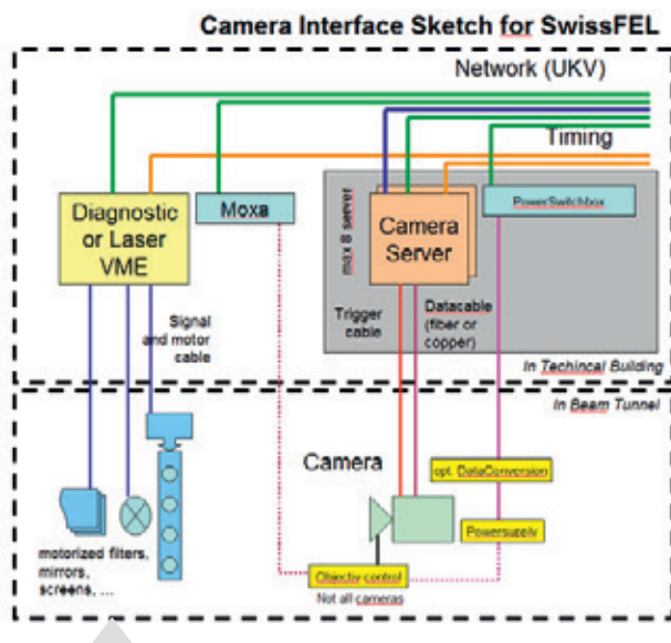
Figure 3.9.5: Camera interface for SwissFEL.
