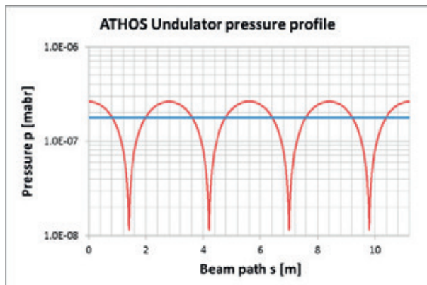
Figure 3.7.2: Pressure profile over 3 vacuum sections of ATHOS undulators.
