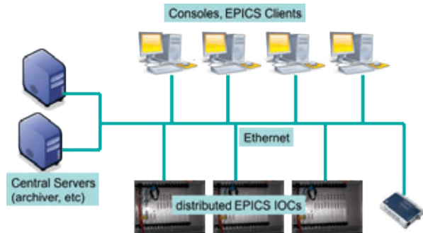
Figure 3.9.1: Control system architecture.
