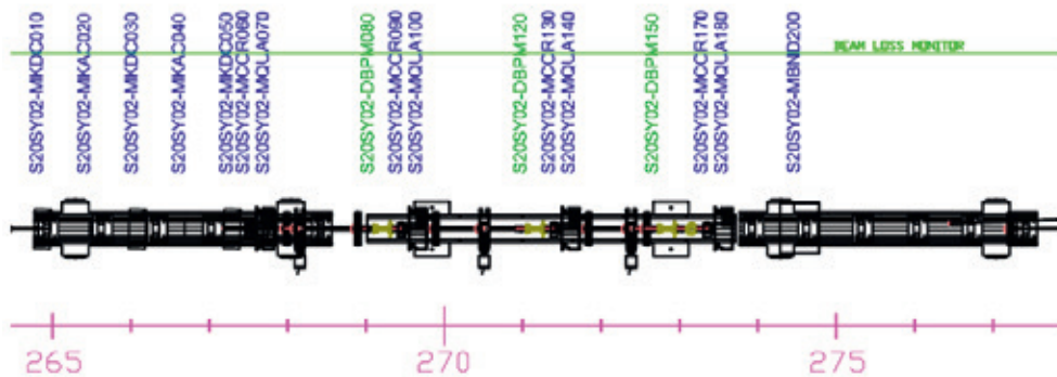
Fig. 3.4.6.1. Kicker and septum layout, with intervening quadrupoles.
