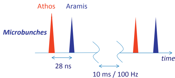
Fig: 1.4.1 Time structure of linac beam.
