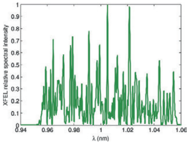
Figure 2.14: Example of a simulated spectrum for an XFEL pulse with a total bandwidth of 10%. It is obtained with a tilt amplitude in offset of 125 and a TGU gradient of 48 m -1 .
