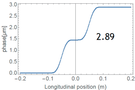
Figure 3.5.4.4: Cumulated path delay (2.89 μm) of the electrons over a straight trajectory (RADIA simulation).
