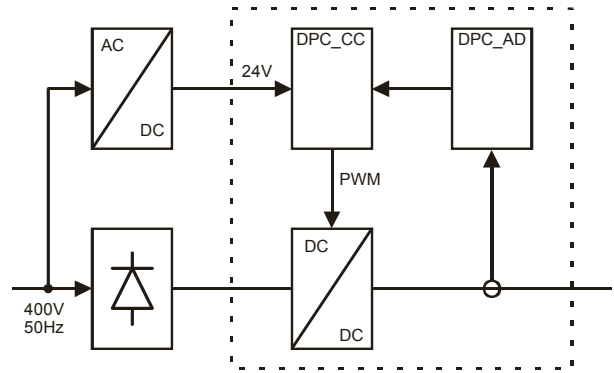
Fig. 3.4.5.3: Converter concept 150.....220A.
