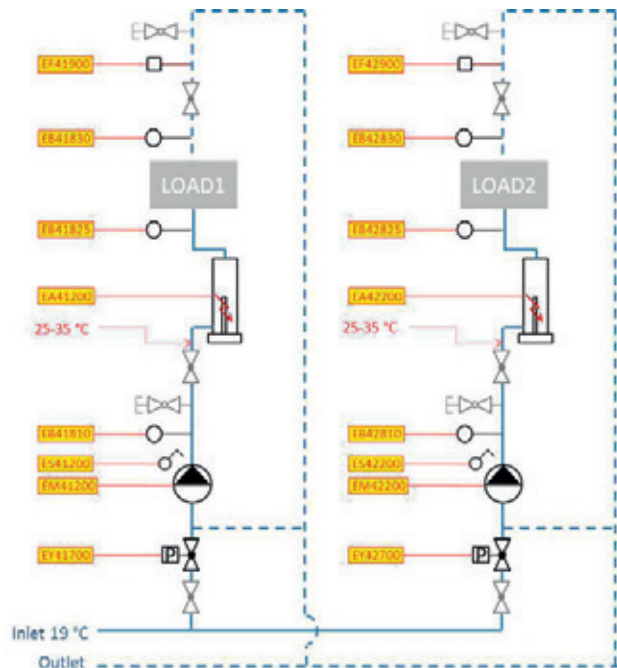
Fig. 5.3.2.2: Principle layout for sub-distribution module „RF accelerating cavities”. Example with two independent cavity sub-distribution circuits within one cooling station.
