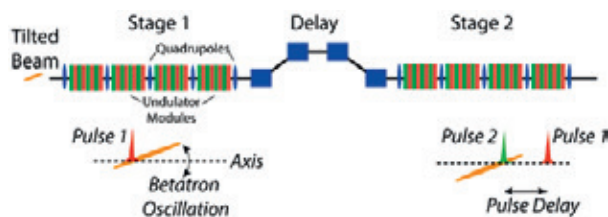
Figure 2.11: Schematic configuration of two color operation.
