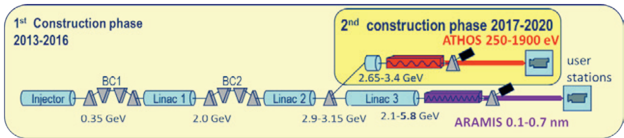
Fig. 1.2.3: SwissFEL layout schematic with the Aramis and Athos FEL.
