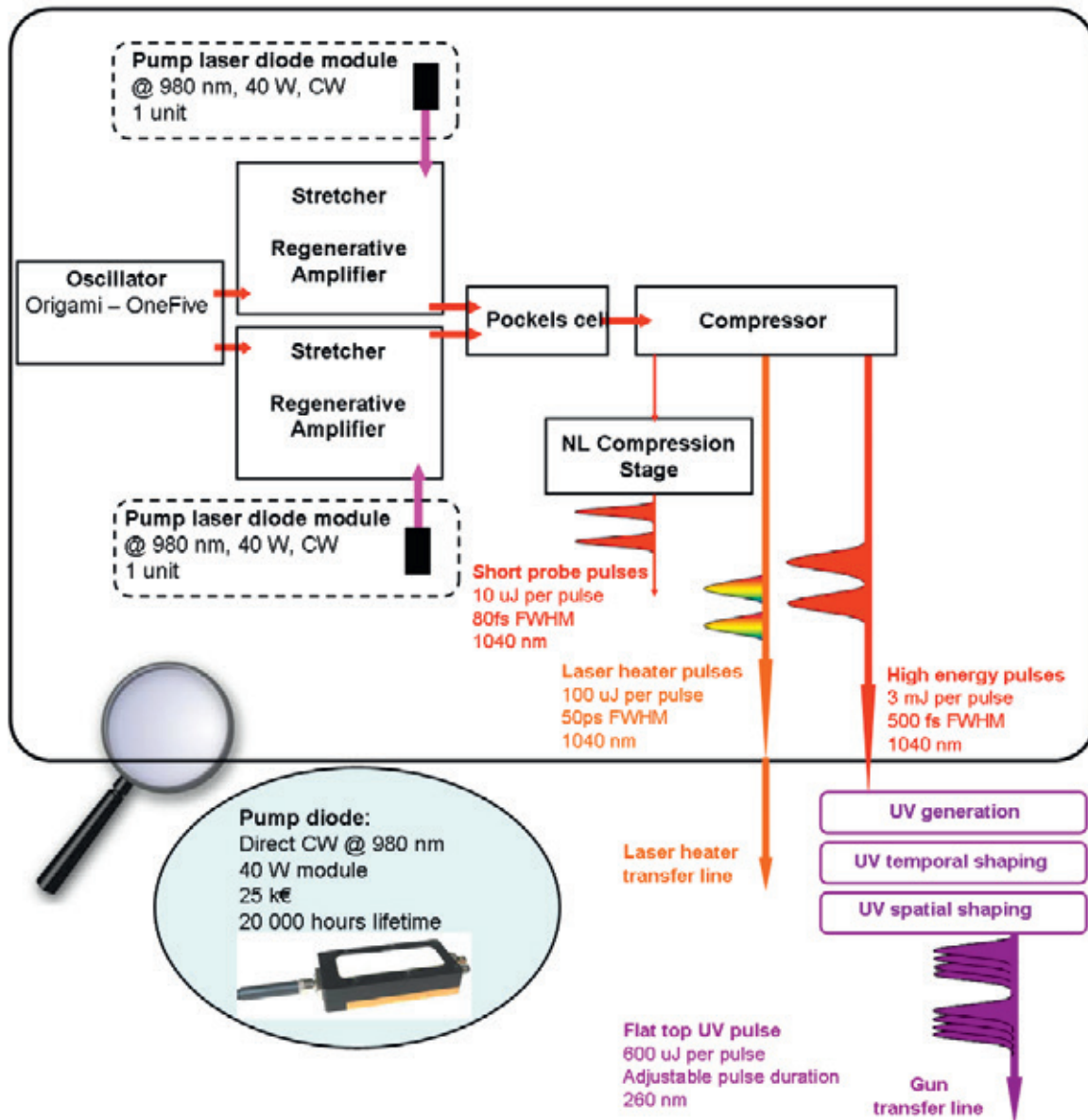
Fig. 3.1.1: Schematic of the gun laser architecture [22]. The system is able to deliver the temporally shaped UV pulses to the gun cathode but also the laser heater pulse and a short probe for UV pulse diagnostic. The system is able to deliver 2 pulses delayed by 28 ns in order to seed the hard and soft X-ray line of the FEL.
