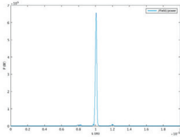
Figure 2.19: Radiation pulse at undulator exit.
