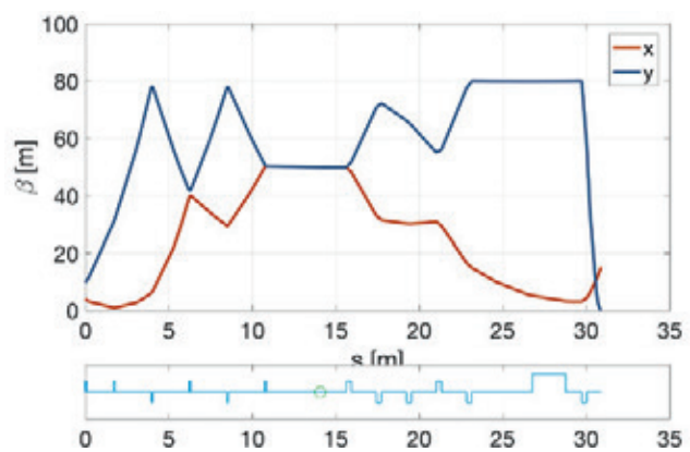
Figure 3.2.3.2: The \beta -function of the beam lattice optics for the post-undulator diagnostic section. s=0 corresponds to the end of the last Athos undulator. The locations of the deflectors are highlighted with a green circle and the \beta_x = \beta_y = 50 m.
