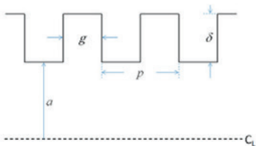
Fig. 3.8.2.2: Generic profile of the corrugated structure (parameters are given in Table 3.8.2.3).
