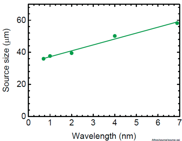
Figure 4.3.2: Rms-values for source size (left) and beam divergence (right) of the Athos-FEL-beam according to Table 4.3.1. A linear regression to the data is plotted in both diagrams. The dashed line in the right diagram shows the divergence of a gaussian beam with the same beam waist as the FEL-beam.
