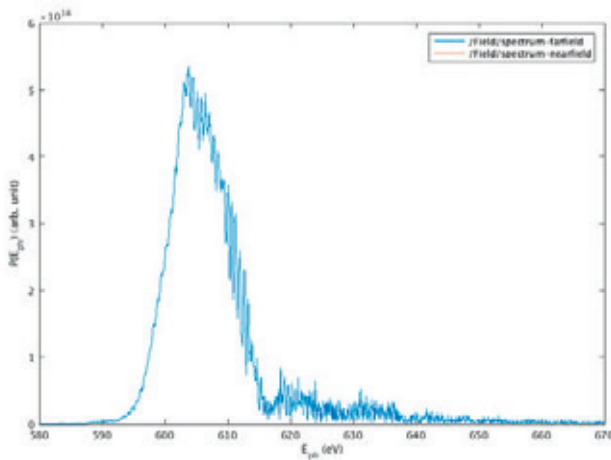
Figure 2.20: Spectrum of FEL pulse at undulator exit.
