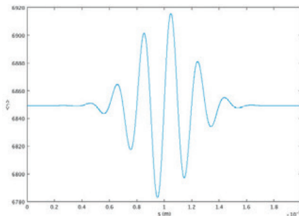
Figure 2.17: Energy modulation of the electron beam at the undulator entrance.
