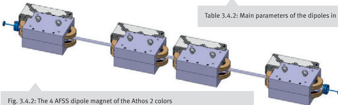
Fig. 3.4.2: The 4 AFSS dipole magnet of the Athos 2 colors chicane to adjust the delay between the two FEL pulses from 0 to 500 fs.
