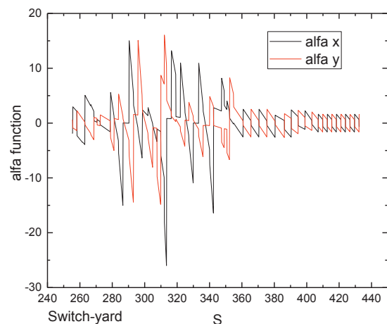
Figure 2.4: Beam optic alfa function of the Athos lattice starting from the switchyard.
