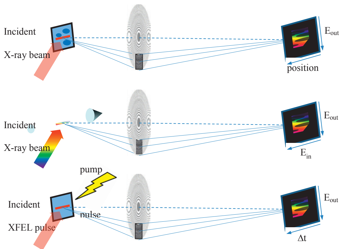
Fig. 4.4.2. Examples of simultaneous measurements that can be performed using off-axis zone plates.
