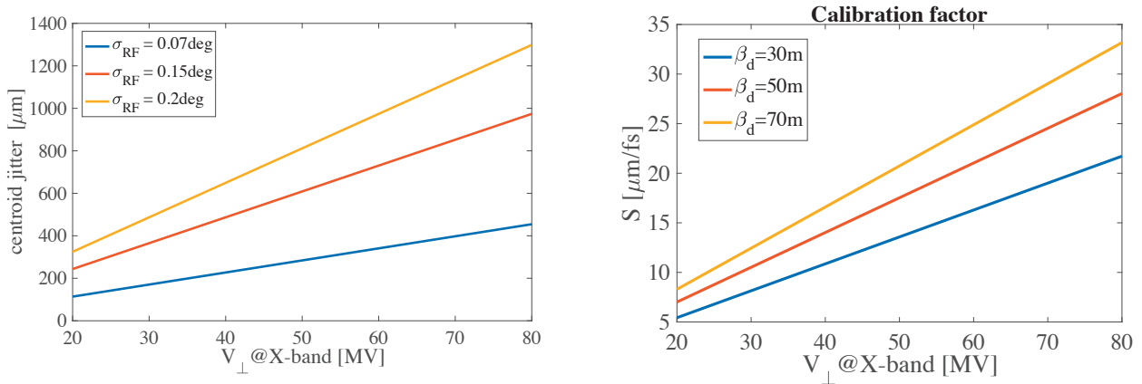
Figure 3.2.3.4: Centroid jitter (left) and calibration factor (right) as a function of the integrated deflecting voltage. Centroid jitter is estimated considering three different values of the RF phase jitter for \beta_d = 50 m.
