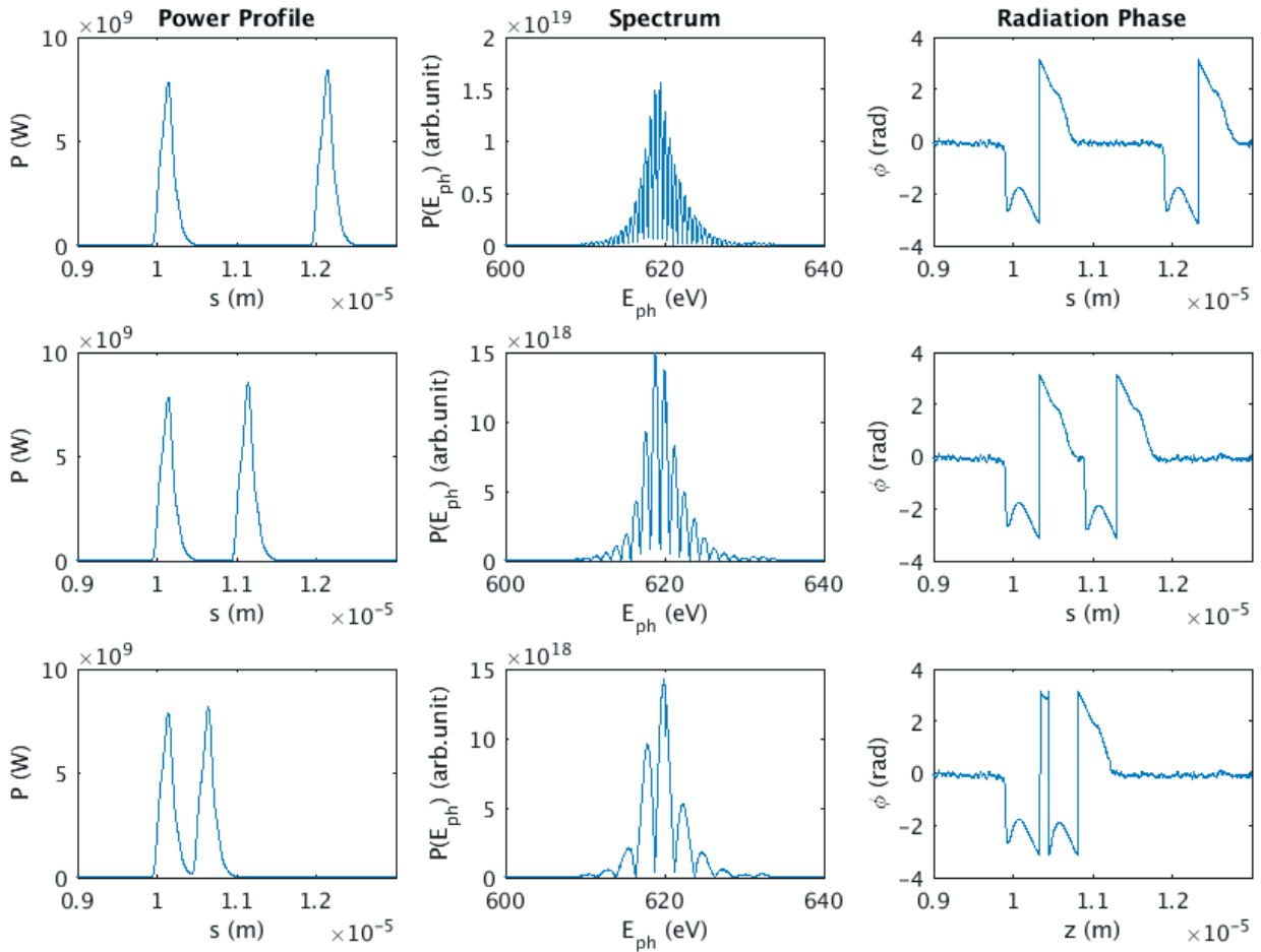
Figure 2.9: Power profile, spectrum and radiation phase (left to right plot) for various separation of the two pulses.
