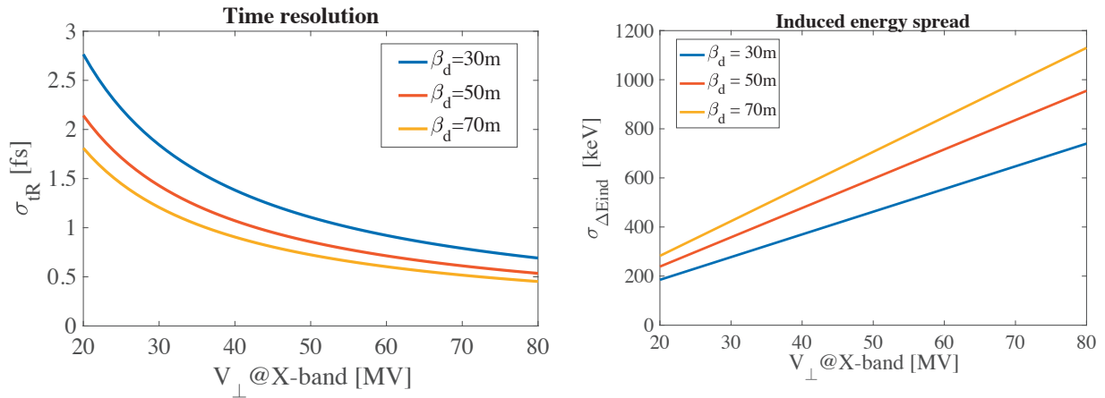
Figure 3.2.3.3: Time resolution (left) and rms induced energy spread (right) as a function of the integrated deflecting voltage. Sub-fs resolution with V_{\perp} \geq 45 MV and \beta_d = 50 m in both transverse planes.
