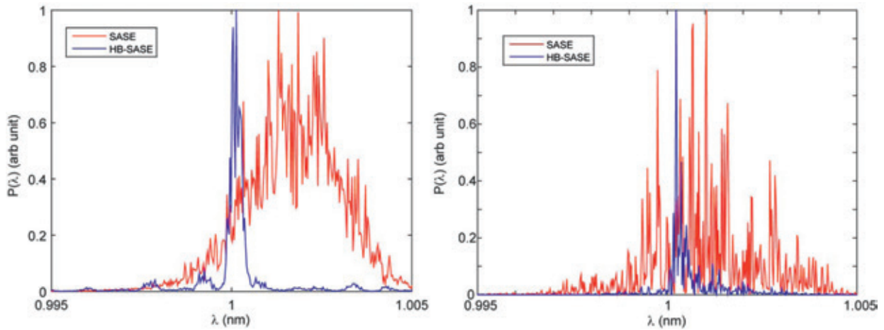
Figure 2.10: Output spectra for an undulator length of L=1.5 m in SASE operation or in the high brightness SASE mode averaged over 10 pulses (left) and for a single shot (right). [12]
