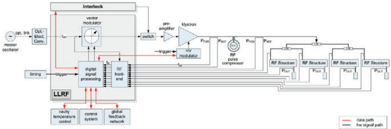
Figure 3.2.4.1: RF system overview of one RF station in the main linac with RF pulse compression.
