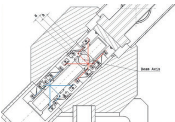
Fig. 3.6.2.2: View of the Transverse section of the WSC vacuum chamber and, in particular, of the wire-fork and of the CF16 vacuum chamber. The wire-fork is equipped with 3 different pin-slots where the wire can be stretched. The distance of the “wire-vertex” from the vacuum-chamber axis can be set at 8, 5.5 and 3 mm in correspondence of the 3 different pin-slots.
