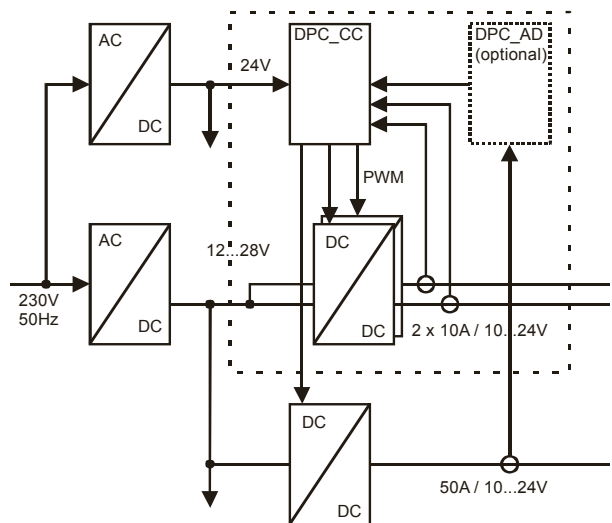
Fig. 3.4.5.2: Converter concept 1*50A+2*10A.
