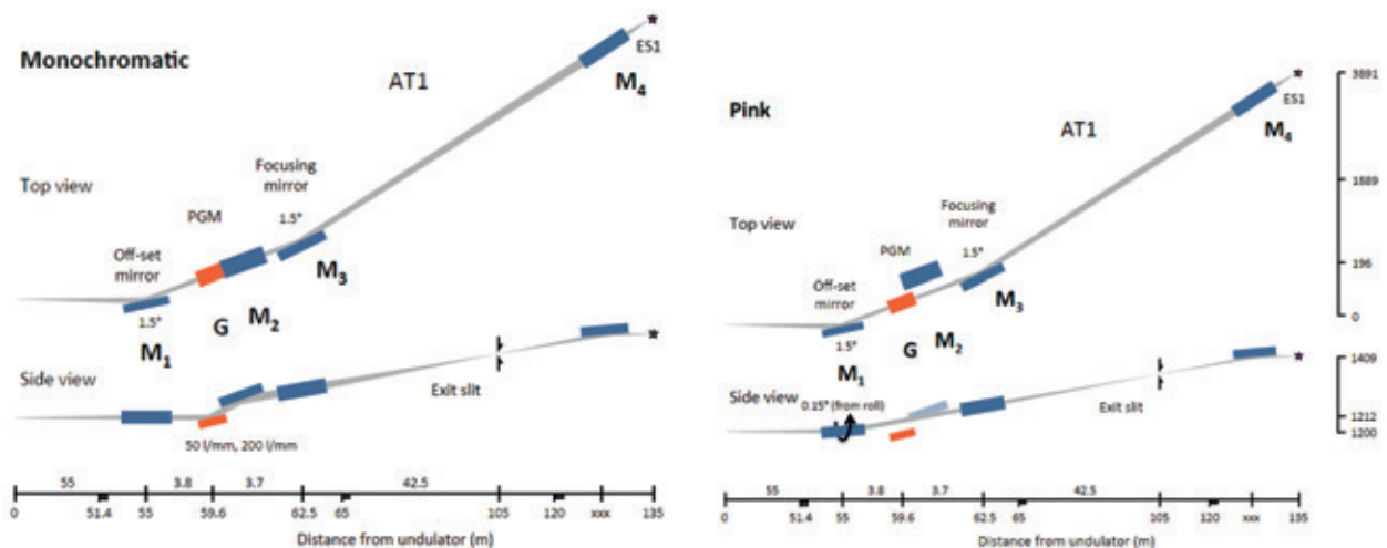
Figure 4.3.5: In monochromatic mode, the first mirror directs the beam horizontally to the plane mirror M2 (shown left). In pink mode, a roll motion of M1 steers the beam in a way that the fix point is hit.
