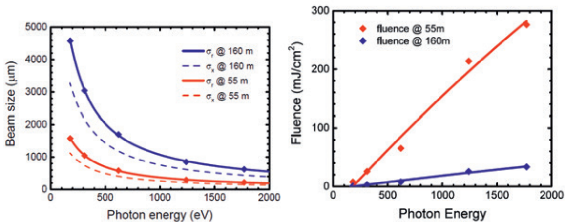
Figure 4.3.3: Left panel: Beam size at the offset mirrors (55 m) and the location of the refocusing mirrors of Athos 3 (160 m). Solid lines are fits to the values of Table 4.3.1, dashed lines represent the projected values according to eqn (4). The right panel shows the peak fluence at the two distances as function of the photon energy.
