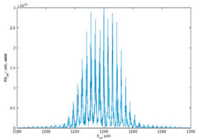
Figure 2.25: Corresponding spectrum of mode-locked pulse.
