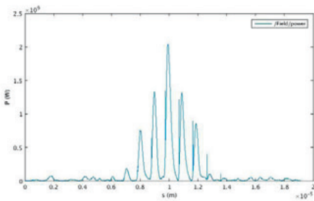
Figure 2.22: Radiation power profile after 5 undulator modules.
