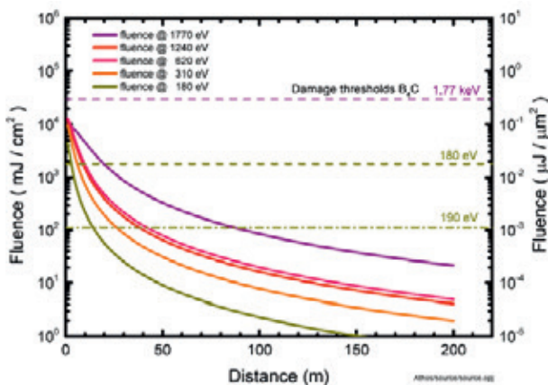
Figure 4.3.4: Fluence along the beamline.
