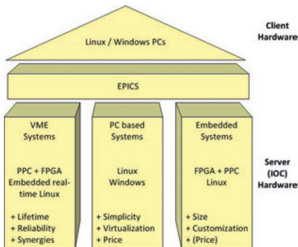
Figure 3.9.2: The three pillars of the SwissFEL/Athos control system.
