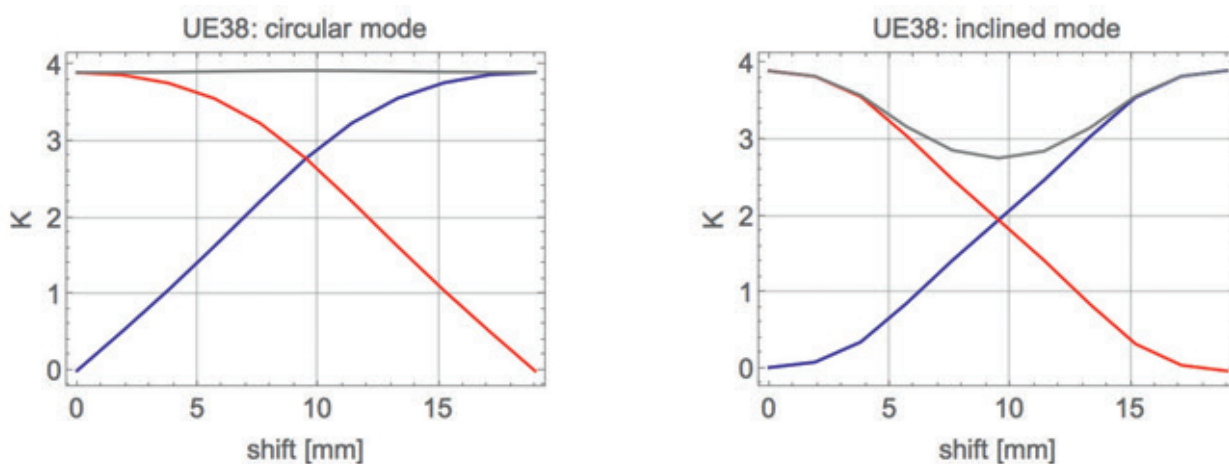
Fig. 3.5.3: K value in the horizontal direction (blue) and the vertical direction (red) and the sum (black) versus the longitudinal shift of the magnet arrays. In circular mode, bottom-left and top-right arrays are shifted by a quarter magnet period in respect to bottom-right and top-left-arrays. In inclined linear polarization, bottom-left and top-right are shifted in opposite direction while other two arrays stay unchanged.
