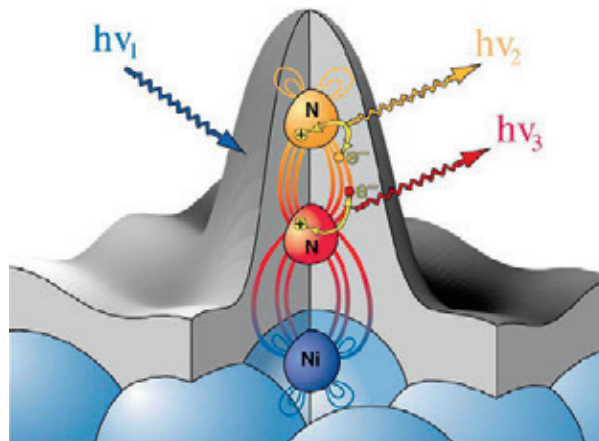
Fig. 1.6.1: Schematic representation of the “local probe” nature of soft X-ray spectroscopy, applied to an N 2 molecule adsorbed on a nickel surface. The grey volume represents the electron density outside the metal surface, and the colored loops indicate a particular molecular orbital, which extends over both nitrogen atoms and a surface nickel atom. Following excitation by an incoming energetic X-rays h\nu_1 , transitions between core and valence electron states, indicated by arrows, produce fluorescence radiation at characteristic photon energies h\nu_2 and h\nu_3 . These transitions are sensitive to the chemical binding of the two nitrogen atoms. The ATHOS beamline at SwissFEL will allow such site-specific probing of electronic binding to be performed in a time-resolved manner after driving the system out of chemical equilibrium, e.g., with an optical laser pulse. The figure is reproduced with the permission of the publisher from A Nilsson and LGM Pettersson, Surface Science Reports , 55, p. 49 (2004).
