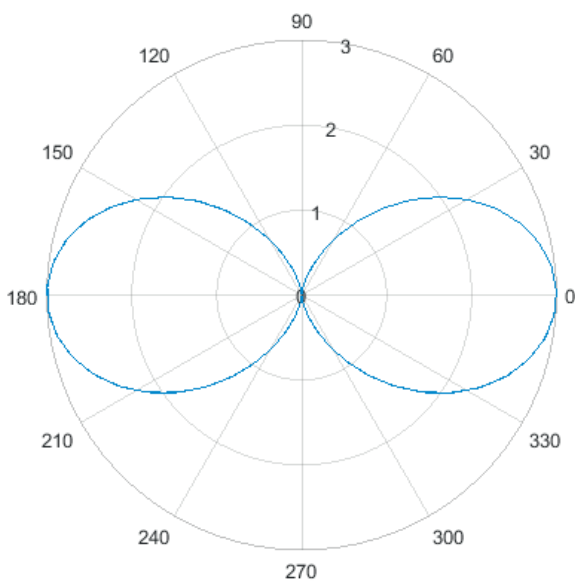
Figure 4.2.2: Angular distribution for s-electrons.
