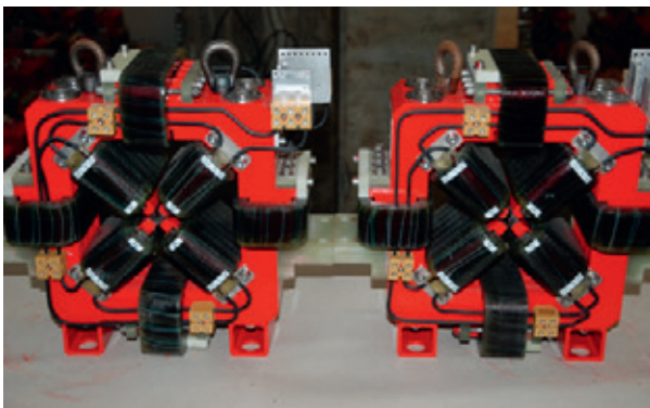
Fig. 3.4.1: QFF quadrupoles from SwissFEL (left picture) with integrated horizontal and vertical steering function. QFM quadrupole from SwissFEL water cooled (right picture).
