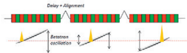
Figure 2.15: Schematic of the tilted beam which is delayed and shifted horizontally at each chicane so that always fresh electrons overlap the XFEL pulse (in yellow).
