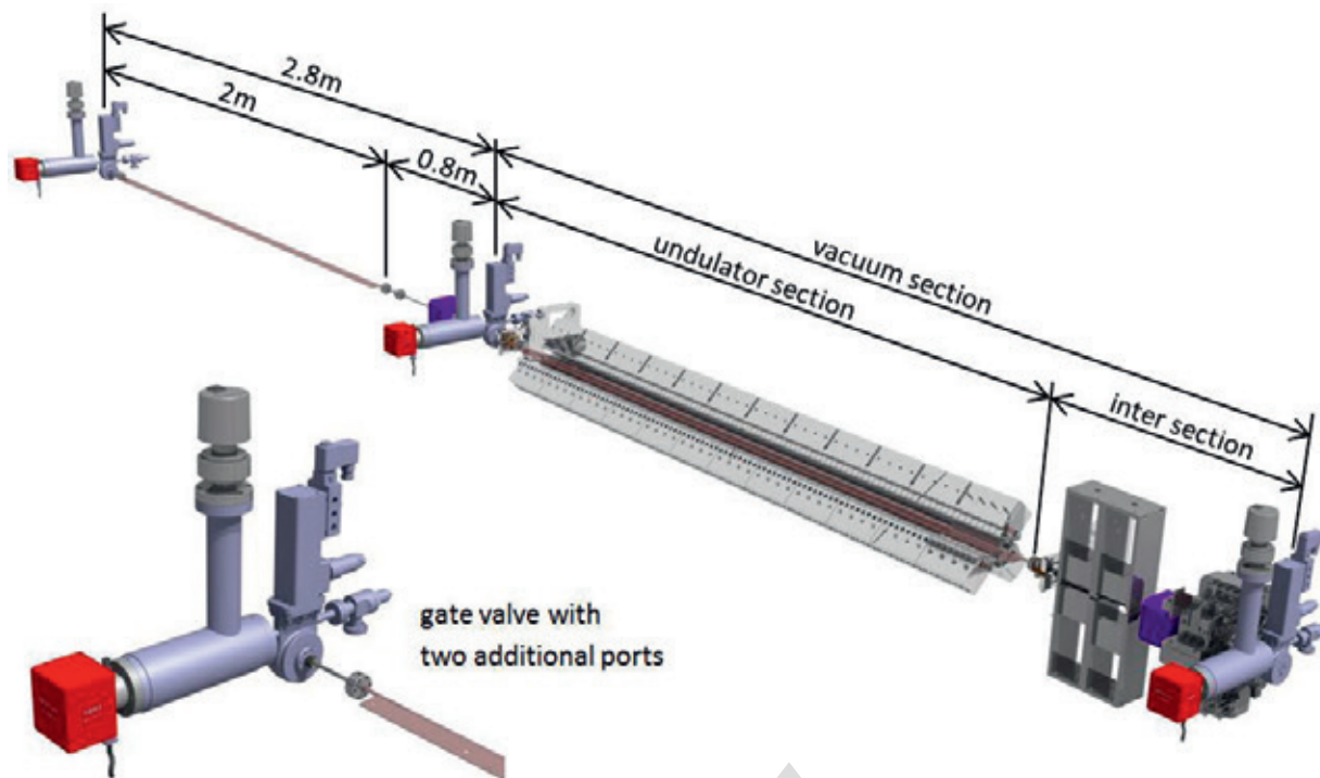
Figure 3.7.1: Arrangement of vacuum components.
