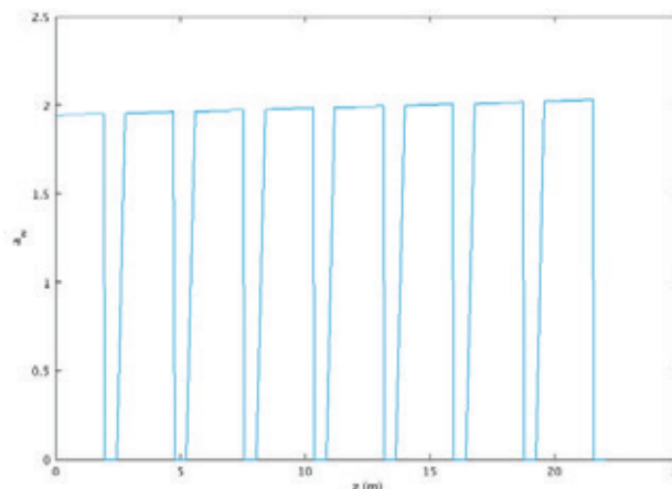
Figure 2.18: Undulator field tapering to preserve resonance for the part in the beam with the largest rising energy chirp.
