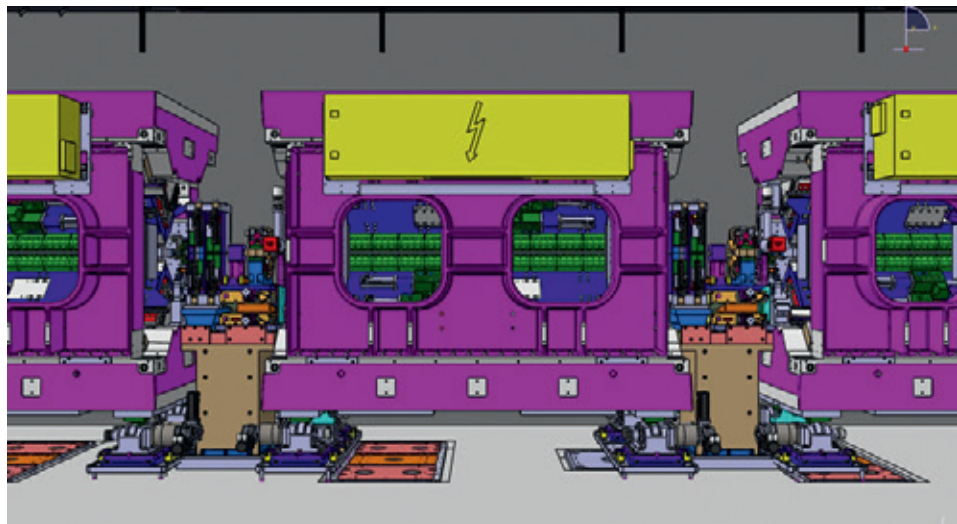
Fig. 3.5.2: Layout of the Athos undulator line: the undulator segment with an inter-undulator section is 2.8m long.
