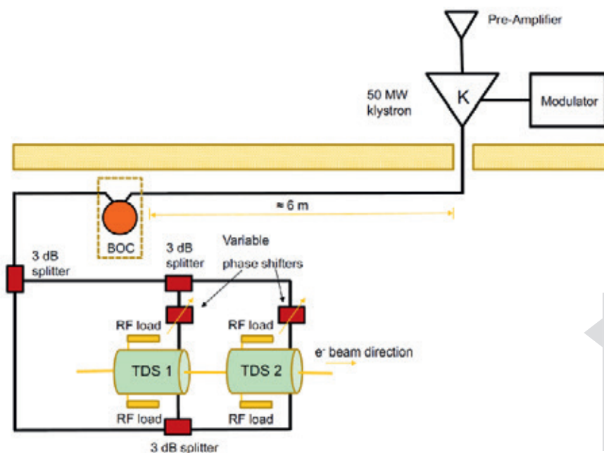
Figure 3.2.3.5: First concept for RF power feeding scheme, with SLED system and waveguide components.
