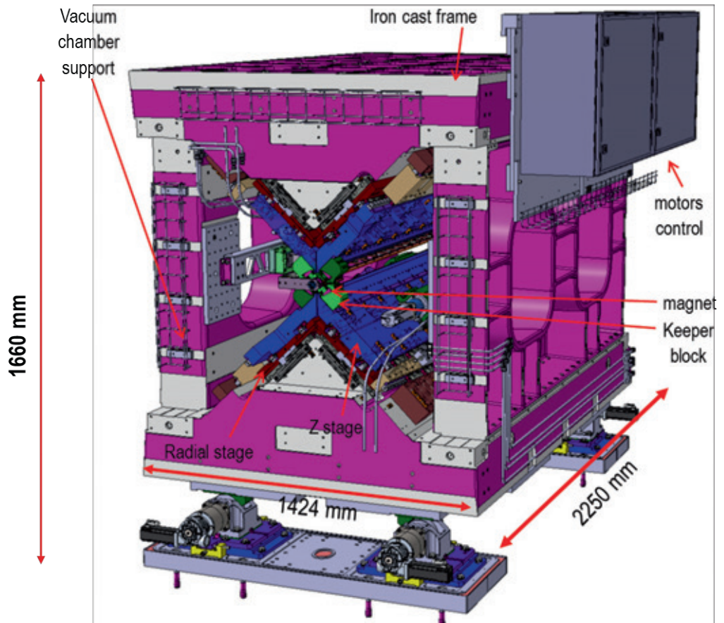
Fig. 3.5.6: Global views of UE38 undulator with reference to the different components.
