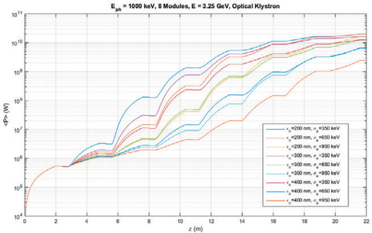
Figure 2.12: FEL performance at 1 keV photon energy for various electron beam parameters.
