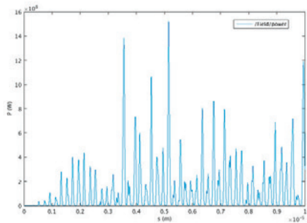
Figure 2.24: FEL profile after 3m of undulator with mode-locked pulse structure.
