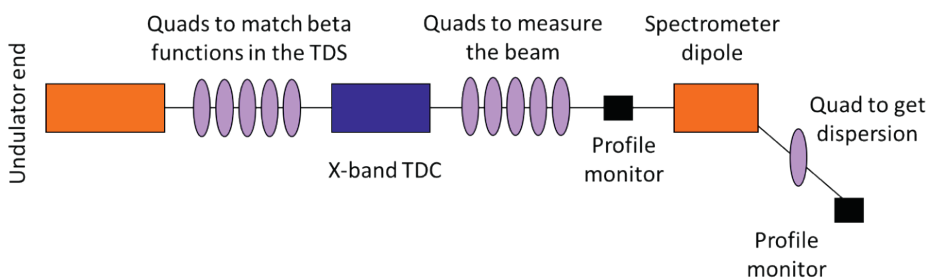
Figure 3.2.3.1: Concept of the post-undulator diagnostic section based on TDS.
