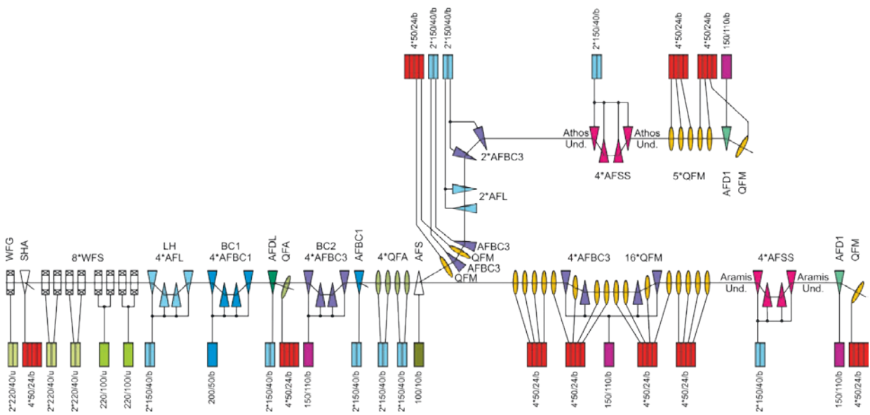
Figure 3.4.5.7: Schematic overview of SwissFEL magnets and power supplies with current ratings of 50A and more.
