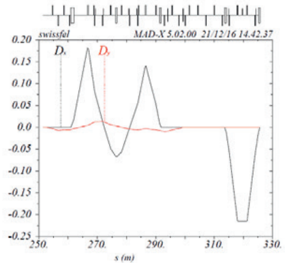
Figure 2.3: Dispersion from S20SY01 to SATCL01 (until energy collimator section).
