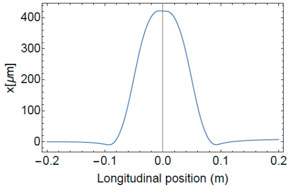
Figure 3.5.4.3: Electron beam trajectory when the gap is closed at 6.5 mm. Electrons deviate by 400 μm in the central two dipoles (RADIA simulation).
