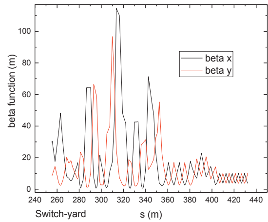
Figure 2.2: Beta function of the Athos lattice starting from the switchyard.
