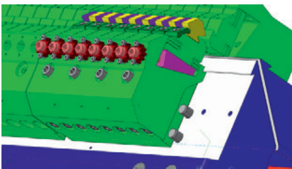
Fig. 3.5.7: 15 cm long block-keeper for 4 periods. The block is partially cut in slices (wire eroded) to allow vertical adjustment of individual pairs.
