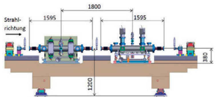
Fig. 3.8.2.3: Preliminary design of the two variable gap/slit dechirper on their girder.
