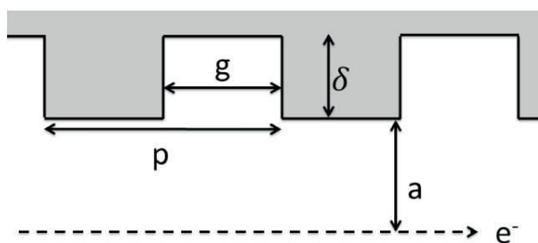
Fig. 2.5: Geometry of a corrugated wall ( p , g , a and \delta have typical values between 0.1 and 1 mm).
