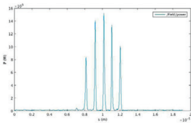
Figure 2.23: FEL signal at 1 nm at saturation after 5 undulator modules in the second stage.
