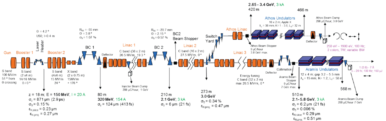
Fig. 2.1: Schematic of the SwissFEL Accelerator and FEL with the simulated beam parameters for the 200 pC operating mode.
