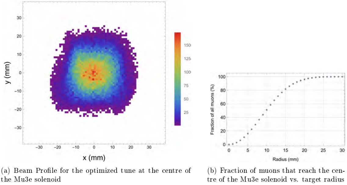
Figure 2.95.: Shown is the beam profile according to the optimized G4BL simulation. The 19 mm target radius contains \sim 95 % of all muons that reach the centre of the Mu3e solenoid.
