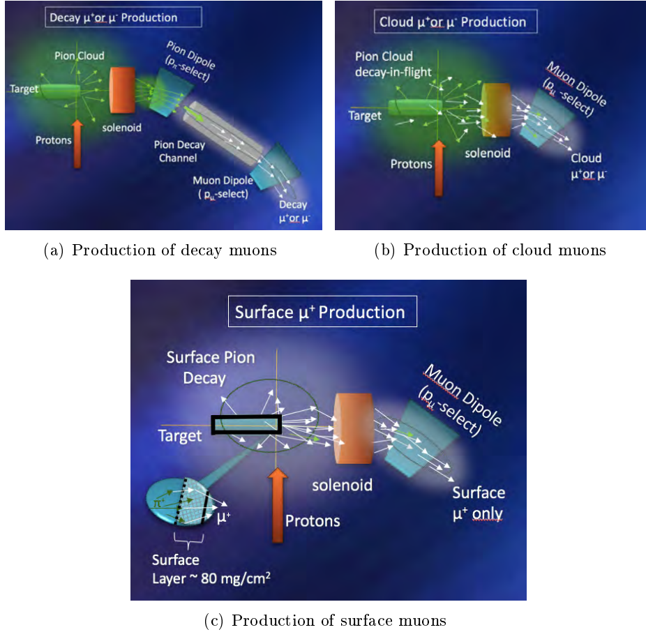
Figure 1.6.: Shown are the different types of muon beams. The figures were taken from [29].
