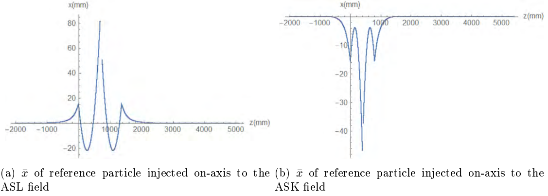
Figure 2.84.: To check the alignment for the positioning that was shown in figure 2.83 the horizontal deviation from the centreline is checked for both magnets. The plots show the horizontal offset \bar{x} of a reference particle that is injected on-axis after being deflected by 90^\circ/65^\circ . The spikes at the magnets' central positions are due to an artefact in the G4BL position reconstruction near a vertex.
