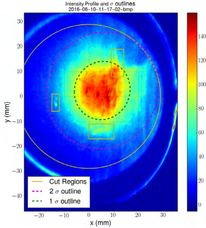
Figure 3.42.: Shown is the corresponding heatplot of the corrected first beam image that was captured on the 10 th of June, after fixing the light leak with an average proton current \bar{I}_{proton} = 2.15 \text{ mA} . The yellow lines indicate the regions of the image that were excluded from fitting.
