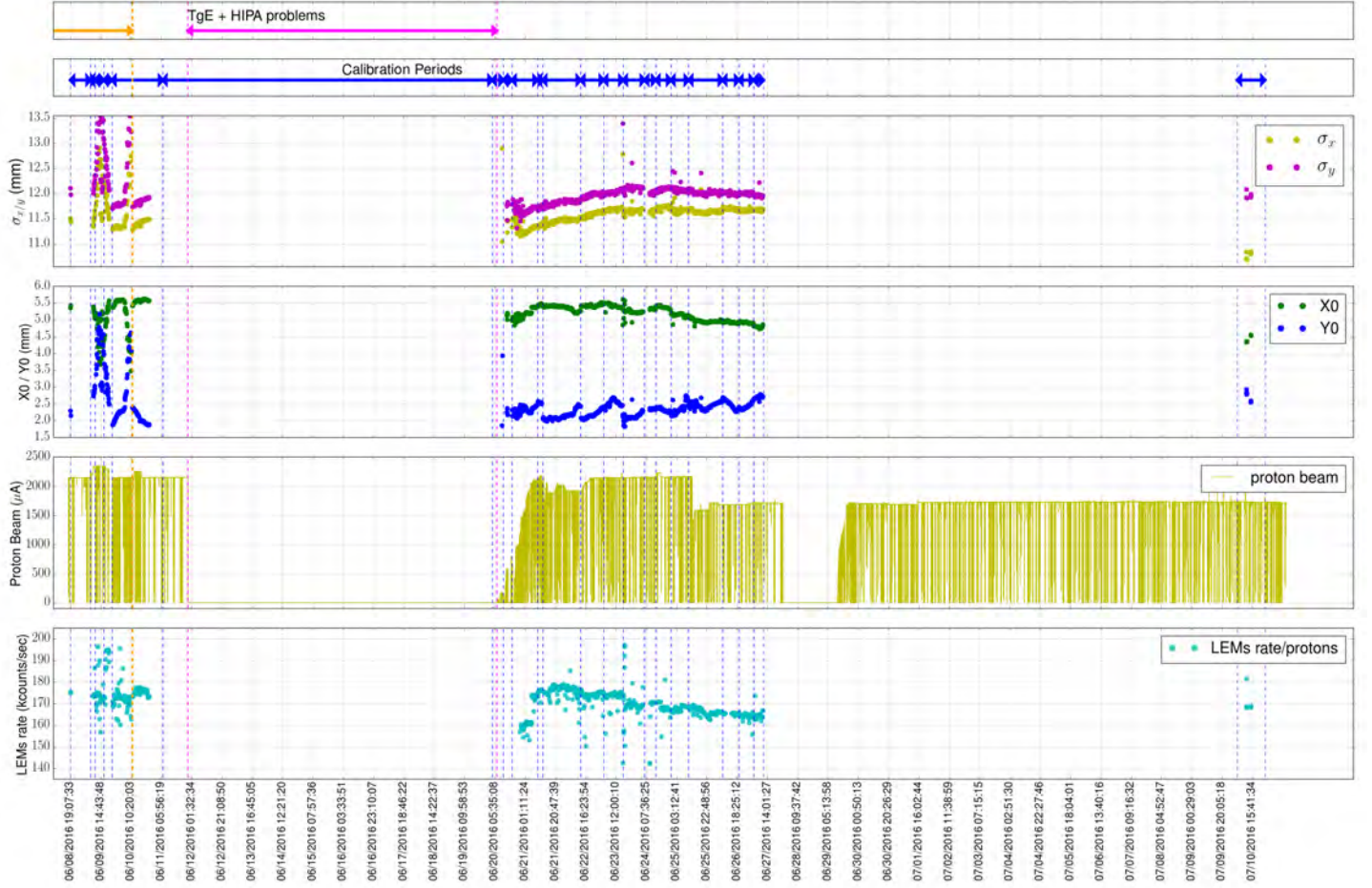
Figure 3.61.: Shown are the beam profile parameters from figure 3.54 with additional data recorded on the 10 th July.
