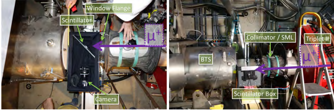
Figure 3.15.: Testbeam setup, the muon beam comes in from the quadrupole Triplet II on the right, passes a collimator system and leaves the beam vacuum through a 190\text{ }\mu\text{m} thin Mylar window. The light tight box containing the scintillator has an aluminum window on the entrance side. The scintillator is mounted with at 45^\circ to the beam axis. The camera views the scintillator also at 45^\circ and perpendicular to the beam axis.
