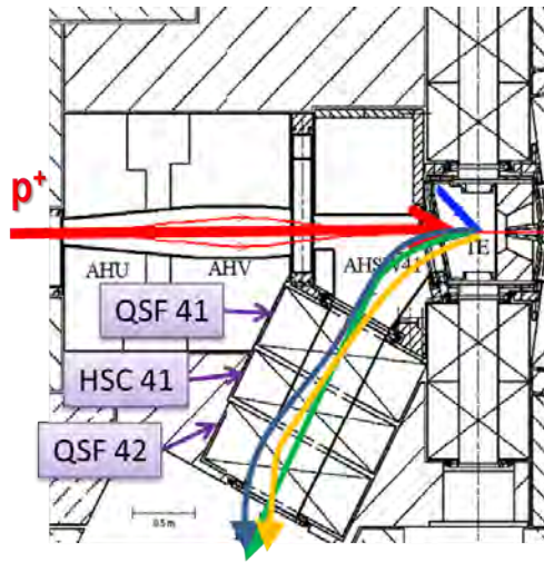
Figure 4.2.: Shown is the muon production target region, the preceeding dipoles in the proton beam line and the first elements of \pi E5. For surface muons the first quadrupole QSF41 after the extraction dipole AHSW is defocussing in the horizontal direction as well as the subsequent sextupole HSC41 although the sextupole is operated at a rather low strength. The QSF42 therefore is horizontal focussing. The centred and parallel design trajectory is shown in green. The blue and the yellow trajectory represent, on the one hand a configuration in which the AHSW is set to provide the correct deflection angle and on the other hand a setting that centers the beam in the QSF41.
