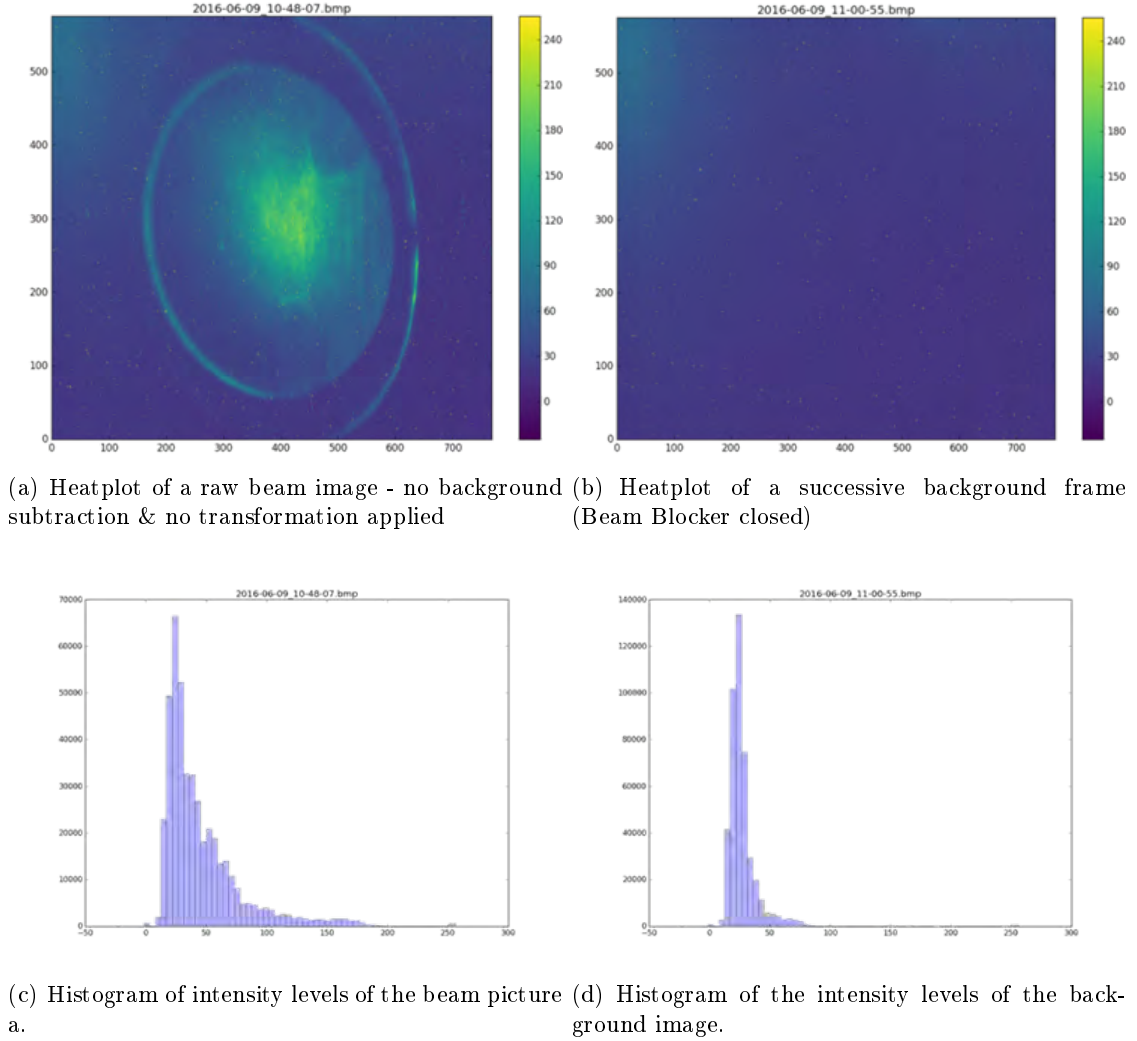
Figure 3.32.: Shown are heatplots and histograms of the ADC levels for a beam and a successive background image. The summed ADC value of all pixels for a raw beam picture amounts to 20300k whereby the sum of all background pixels amounts to 11965k for the same exposure time.
