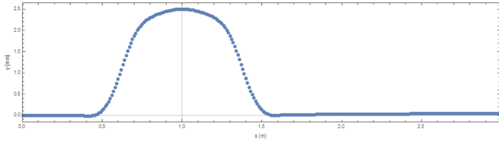
Figure 2.28.: Example of a 10 MeV/c \mu^- starting at s=0 is tracked through the superposition of the separator E -field tuned to 100 kV and the B -field equivalent to 63.2 A coil current, centred at s=1 m. The deceleration on-axis by \sim \frac{100 \text{ kV}}{2} causes the reference particle to leave the central orbit at the injection and come back to the central orbit at the exit.
