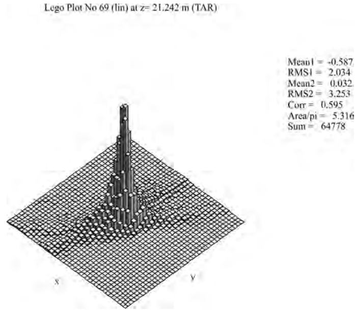
(a) Beam Profile at the target location
