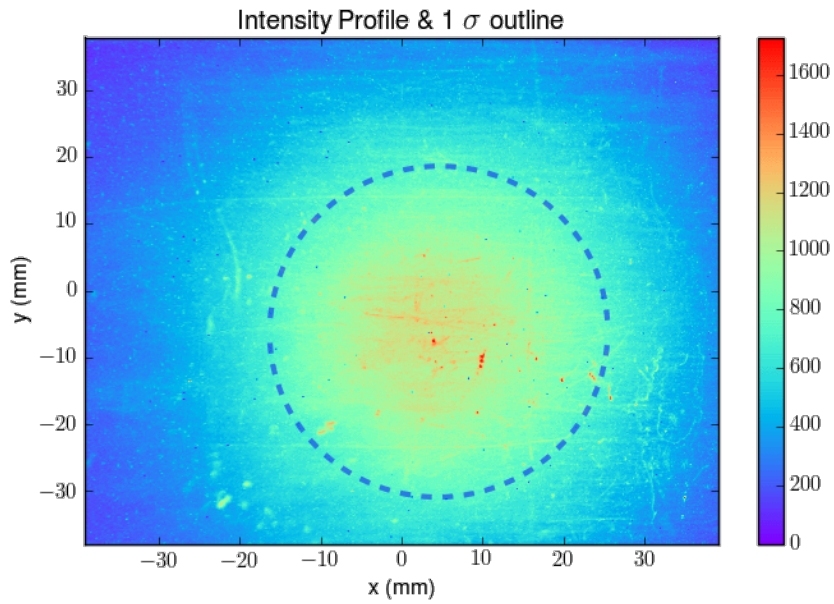
Figure 3.23.: The background subtracted and transformed image is shown together with the 1\text{-}\sigma outline of the fitted distribution. The picture already shows qualitatively that x and y are essentially uncorrelated, consistent with the small xy -coupling throughout the \pi E5 beam line.
