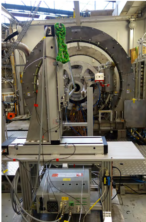
Figure 4.14.: View of the APD scanner from the DS COBRA side. The APD scanner is moved to the measurement position. The endswitches that can be seen on the horizontal and the vertical axis are connected with the interlock connector on the controller box underneath.
