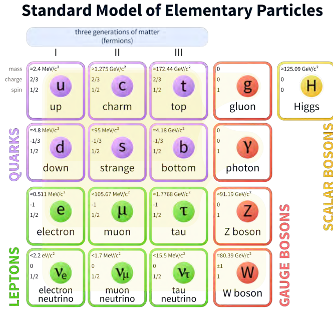
Figure 1.1.: Overview of the fundamental particles in the SM [9]
