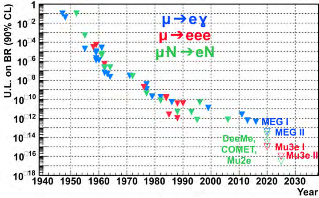
Figure 1.3.: History of cLFV upper limits on the golden channels. The plot is adapted from [24]
