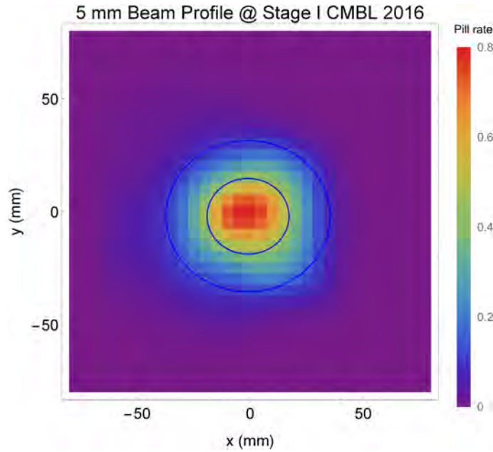
Figure 2.85.: The beam line was optimized for the Pill1 position. The raster scan and a 2D Gauss fit yield the following parameters: \bar{x} = -0.94 \text{ mm} , \bar{y} = -2.08 , \sigma_x = 18.12 \text{ mm} , \sigma_y = 16.73 \text{ mm} , \rho_{xy} = 0.0016 . The rate according to the scaled sum of all measurement points is 1.11 \cdot 10^8 \mu^+/\text{s} @ 2.2 mA proton current
