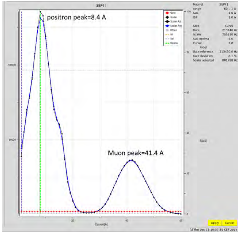
Figure 2.67.: Shown is a low threshold separator scan at the final focus position. The separator magnet currents are varied and the combined rates of both \mu^+ and e^+ are measured on the centreline.
