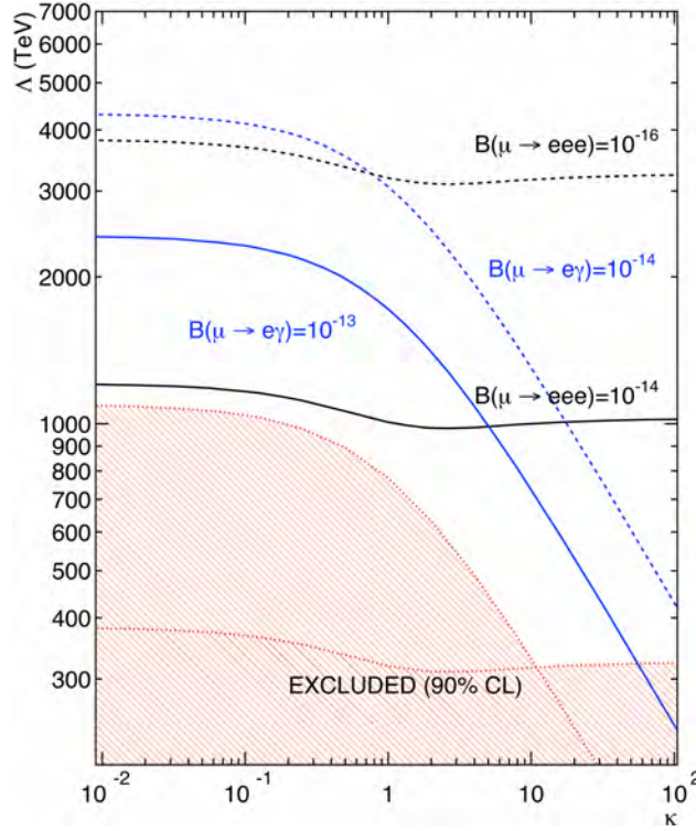
Figure 1.5.: [25] The plot illustrates the high energy scales which can be tested in a model independent way by searching for the cLFV decays \mu^+ \rightarrow e^+ + e^+ + e^- and \mu^+ \rightarrow e^+ + \gamma using an effective field theory approach. For smaller \kappa values (dipole interactions) \mu^+ \rightarrow e^+ + \gamma measurements are sensitive to much higher energies than \mu^+ \rightarrow e^+ + e^+ + e^- . Conversely new physics that is dominated by four-fermion interactions (higher \kappa values) is much more likely to be discovered by \mu^+ \rightarrow e^+ + e^+ + e^- experiments.
