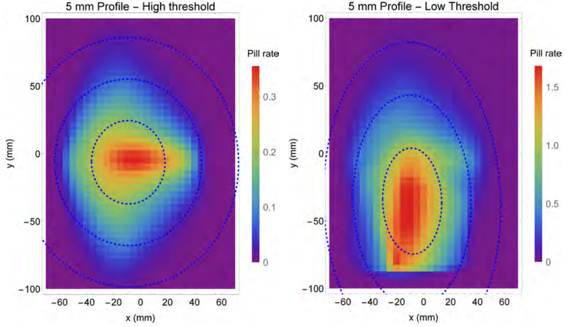
(a) Raster scan of muons only at the Pill1 position (b) Raster scan of the combined rate of muons and positrons at the Pill1 position with the inner collimator removed
