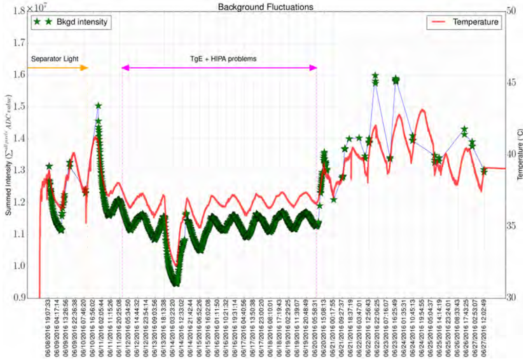
Figure 3.36.: The summed ADC values of the background images show significant fluctuations over time. However the temperature sensor mounted on the iDS camera housing shows a clear correlation with the background intensity levels.
