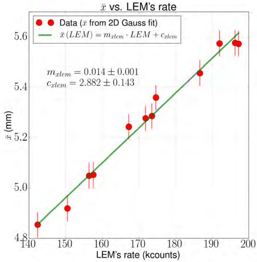
Figure 3.51.: Shown is the relationship between the centroid of the muon beam Gauss fit result from the scintillation target and the normalized \frac{LEM}{I_{p+}} rate which is a linearly measure of the proton beam centring on TgE. The reduced \chi^2 is \frac{\chi^2}{d.o.f.} = 0.36 .
