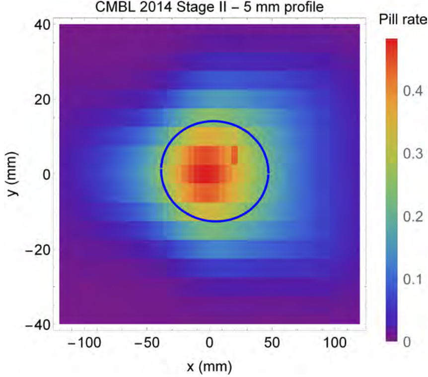
Figure 2.62.: A 2D Gauss fit of the raster scan, that was taken at the end of the stage II beam tuning in the 2014 CMBL beam time yields: \bar{x}=4.11 mm, \bar{y}=0.76 mm, \sigma_x=42.84 mm, \sigma_y=13.33 mm, \rho_{xy}=0.023 and a rate of 6.03 \cdot 10^7 \mu^+/\text{s} at 2.2 mA proton current.
