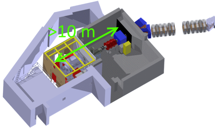
(a) Distance between camera and separator \gtrsim 10 m.
