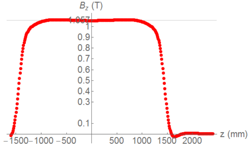
Figure 2.34.: The effective length of the Mu3e solenoid fieldmap based on field calculations [67] for a realistic configuration is given by l_{eff} = \sim 2828 mm / 2806 mm (normalizing to the field at the centre/maximum field)
