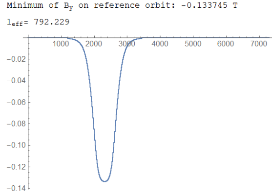
Figure 2.82.: Shown is the B_y field that is "seen" by the reference particle in figure 2.81. From this the effective length is extracted as l_{eff,ASK,first\ try} = 792.2 mm.
