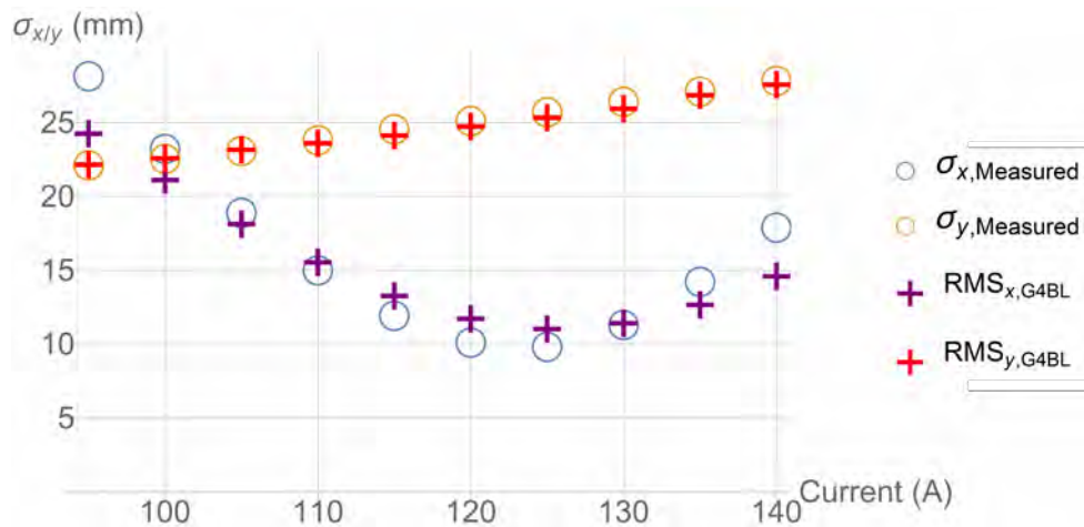
Figure 2.76.: The QSM in the G4BL simulation was tuned to the same current values as for the phase space measurements in the experimental area. The plot compares the respective widths for the measurements and the simulation.
