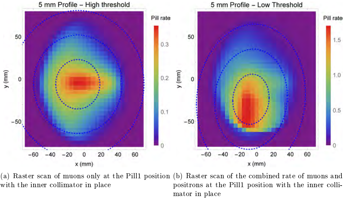
Figure 2.88.: For the shown raster scans at the Pill1 position the collimator was in place. The high threshold scan (left) takes into account only muons and the low threshold (right) also counts Michel and beam positrons. The evaluation of the high threshold scan yields:
