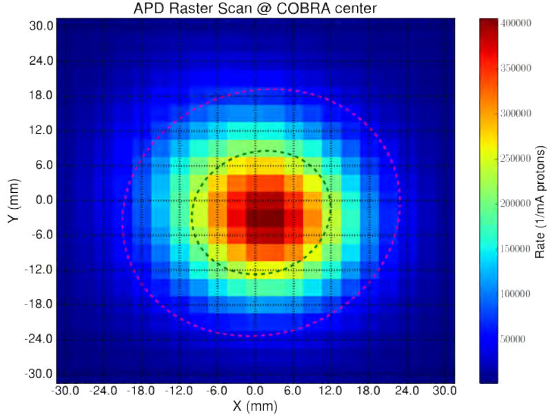
Figure 3.41.: The plot shows the result of the 3 mm APD raster scan measured in a plane perpendicular to the beam direction at COBRA centre. The raster scan yielded 9.16 \cdot 10^7 \mu^+ / s . The profile parameters are listed in table 3.6.
