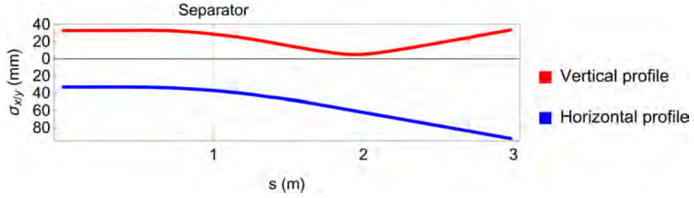
(a) The horizontal and vertical envelopes are plotted for a negative 10 MeV/c muon beam with the separator centred at s=1\text{m}
