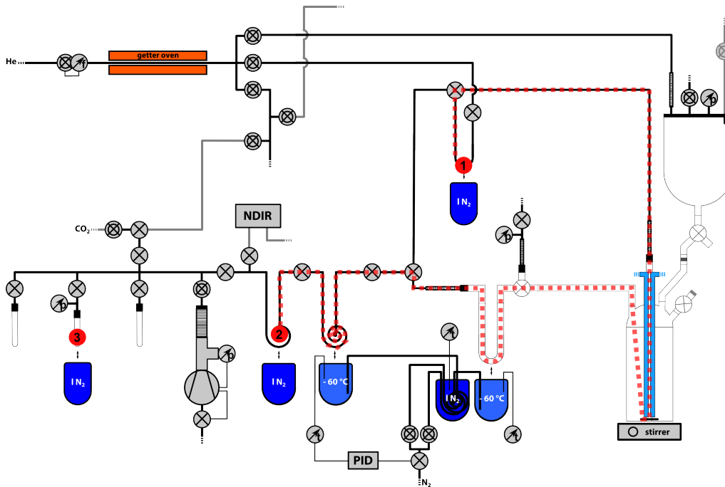
Figure 3.1: Experimental setup to determine the recovery of \text{CO}_2 from the liquid sample. '1': the U-tube is loaded with a known \text{CO}_2 sample, '2': the \text{CO}_2 is transferred through the setup with the helium carrier gas stream (red, dashed line) and captured in the \text{CO}_2 trap. '3': the recovered mass is determined in the manometry cell. The detailed and complete setup is shown in Fig. 2.1.
