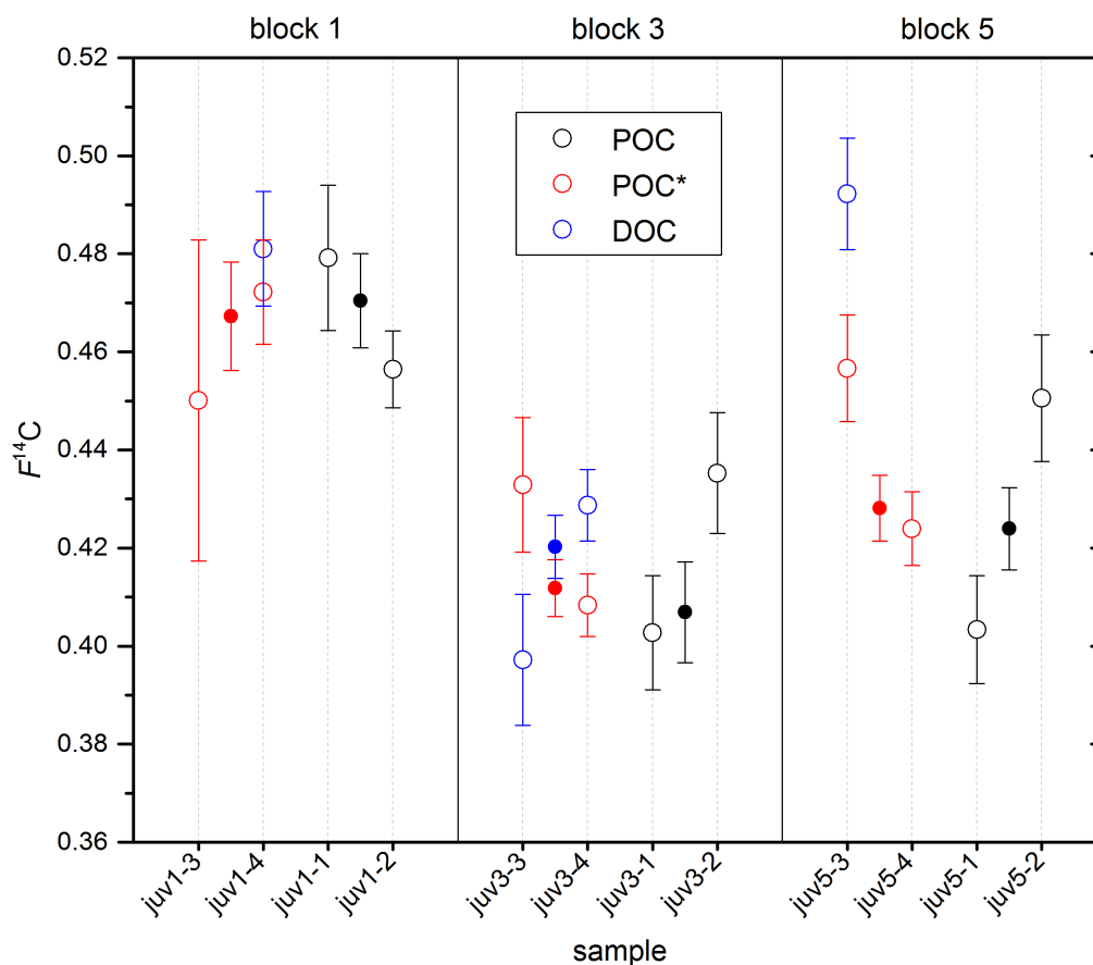
Figure 4.2: F^{14}\text{C} of the validation ice samples from Juvfonne ice tunnel, Norway. From each ice block (1, 3 and 5), four ice samples were taken and analysed for ^{14}\text{C} . Results obtained with the original method for \text{PO}^{14}\text{C} analysis are shown in black with the respective uncertainties. The measurements with our new setup reveal the ^{14}\text{C} content both from POC as well as from DOC as shown in red and blue, respectively. For all samples, open circles represent individual measurements, filled circles the mean value for each ice block and method. Please note the enlarged y-axis (full scale: 0 – 1).
