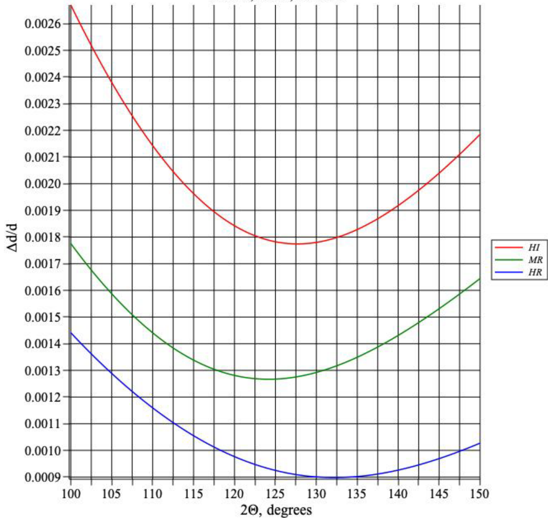
6mm V, 2.45A, delta d/d
