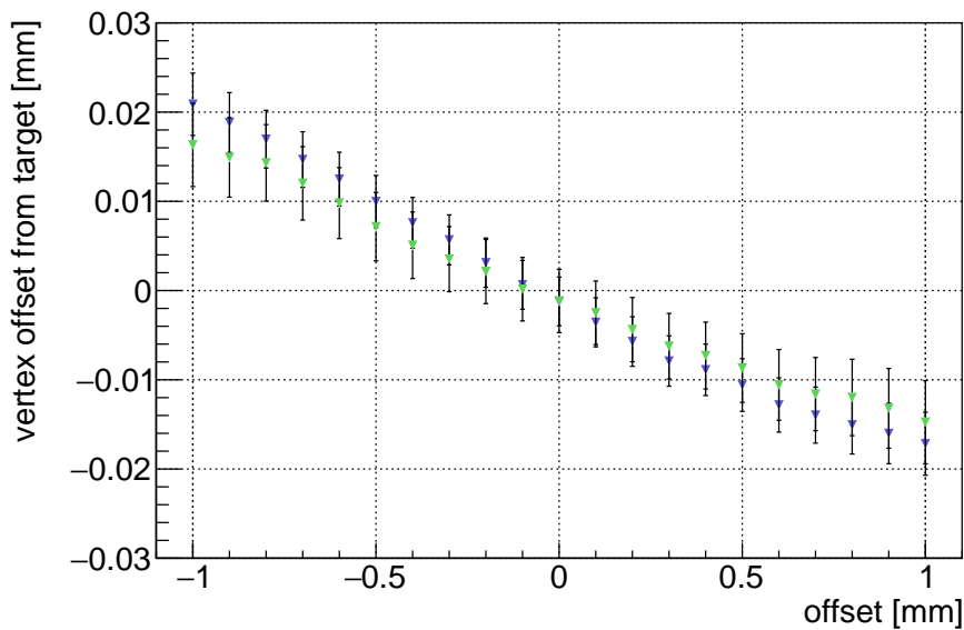
FIGURE 4.5: Three dimensional distance between reconstructed vertex position and target surface for using only long tracks for reconstruction (green) and for all possible tracks (blue). The stated offsets correspond to the systematic misplacement of vertex layer along beam direction.
