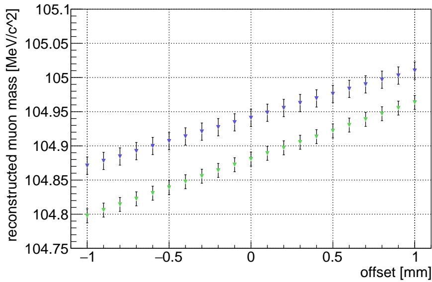
FIGURE 4.4: Reconstructed muon mass as a function of systematic misplacements of the recur stations for utilising only long tracks (green) and for all possible tracks (blue) for reconstruction. The stated offsets correspond to the systematic misplacement of both recur stations simultaneously towards each other (along beam direction). Hence, a negative offset corresponds to a “stretching” and a positive offset to a “squeezing” of the detector.
