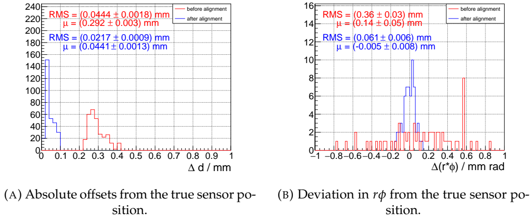
FIGURE 6.7: Offsets before and after two alignment iterations of one pixel layer utilising the hierarchy alignment.
