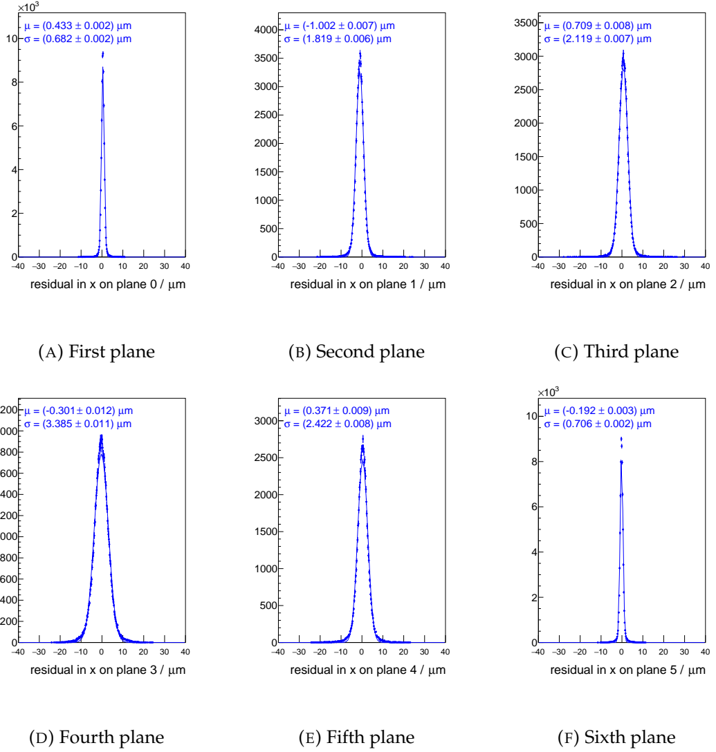
FIGURE F.3: Six-plane EUDET type telescope: Track residuals for an aligned EUDET type telescope in local x-direction. The stated \mu and \sigma are the means and standard deviations of the depicted Gaussian fits.
