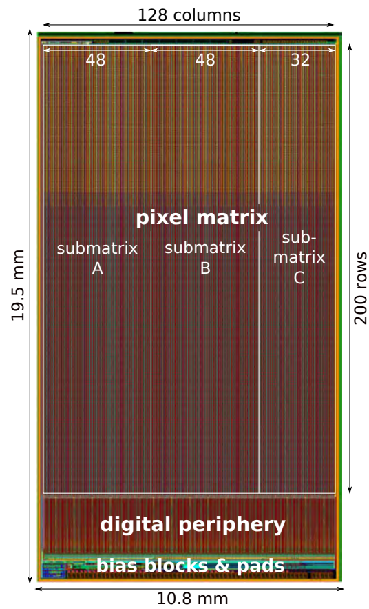
FIGURE 3.4: Layout of the MuPix8 prototype.
