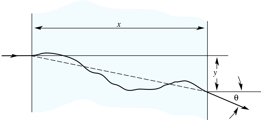
FIGURE 2.4: Multiple scattering of a particle traversing material. The particle is deflected multiple times inside the material which leads to an offset y and a scattering angle \theta with respect to its incoming trajectory. Figure based on [5].
