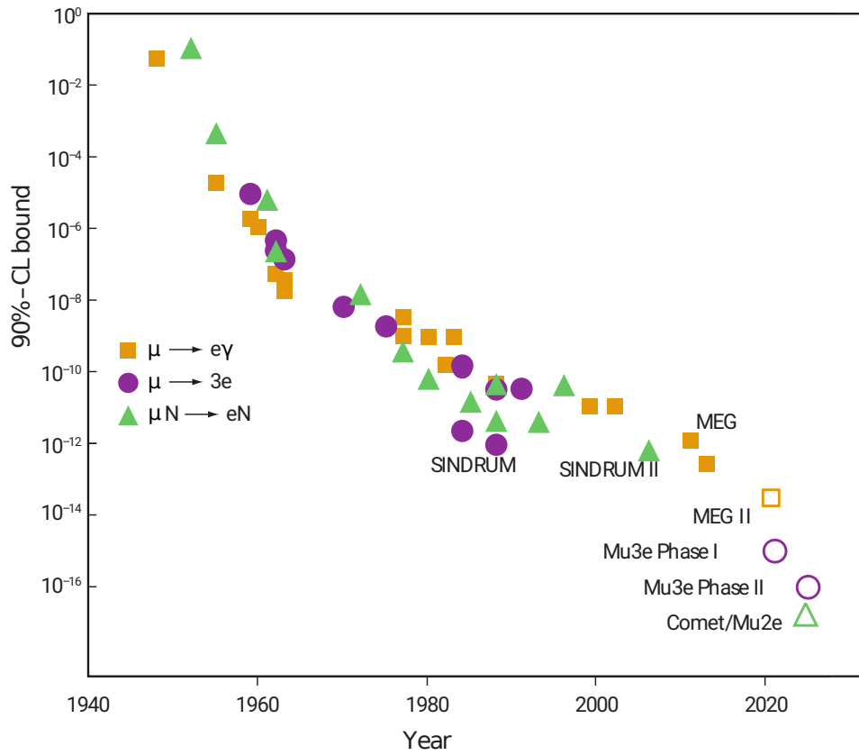
FIGURE 1.5: Past and future experiments searching for lepton flavour violation for muons decaying to electrons. Hollow markers represent future experiments that are under development, solid markers represent currently running or already concluded experiments. Adapted from [12] and updated with recent experiments.
