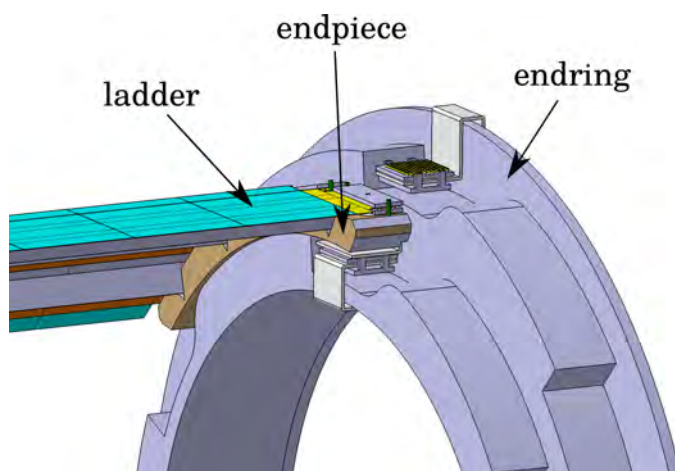
FIGURE 2.11: CAD model of a pixel module mounted with an endpiece onto an endring. Figure based on [15].
