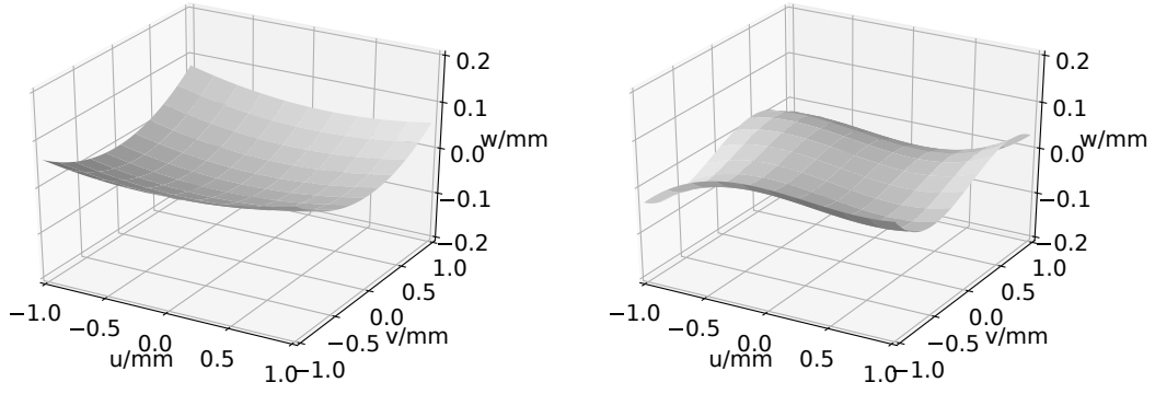
FIGURE 5.6: Example configurations of sensor surfaces parametrised by the height map in Equation 5.21. On the left, Legendre polynomials of up to second order are used, on the right, up to third order. Surface coefficients are of the size of how they are expected after detector construction.
