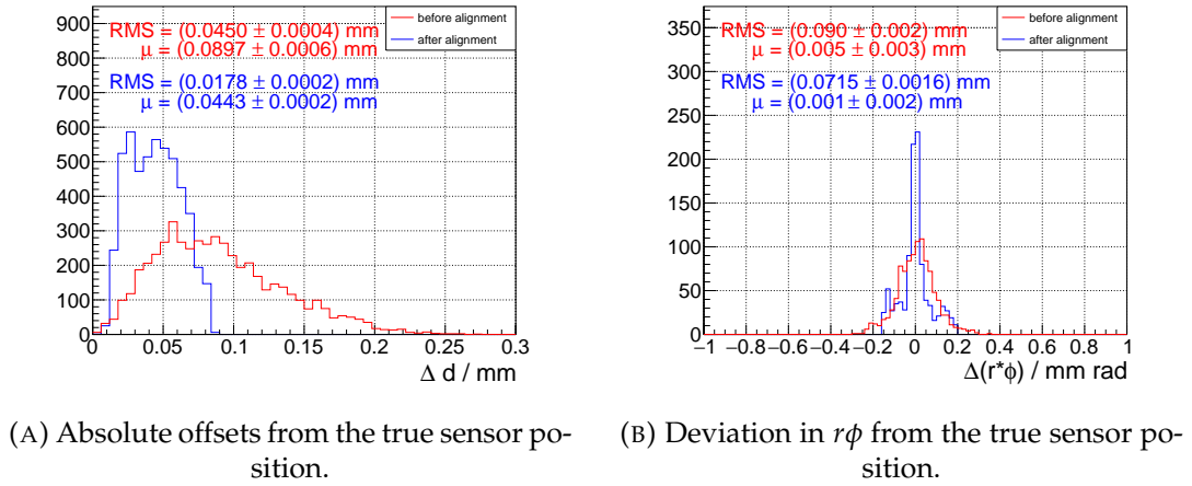
FIGURE 6.4: Offsets before and after alignment of sensor positions and rotations in the central detector station.
