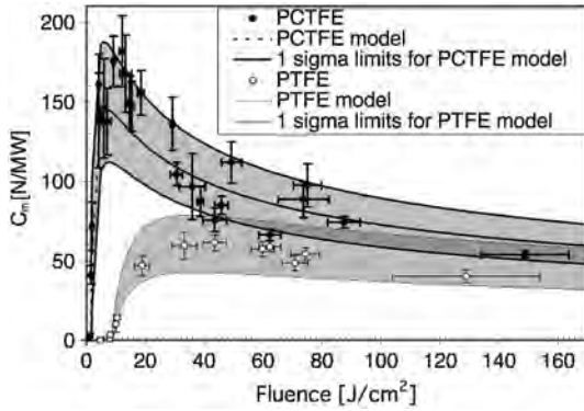
Fig. 11 The Sinko model predicts C_m for pulsed CO 2 -laser radiation C_m on polychlorotrifluoroethylene polymer (PCTFE) below and perhaps slightly into the plasma regime. PTFE denotes polytetrafluoroethylene (Teflon). Modeling limits ( \pm 1\sigma parameter estimates) and experimental error bars ( \pm 1\sigma ) are included. Each point is an average of 5–10 shots (see [70]); used with permission from the American Institute of Physics, copyright 2009.
