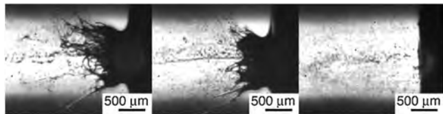
Fig. 15 Pictures taken after 10 \mu\text{s} with 4.5 J/cm 2 for varying GAP concentrations (left to right: 28, 50, and 70%); adapted from a more complete data set in [90].
