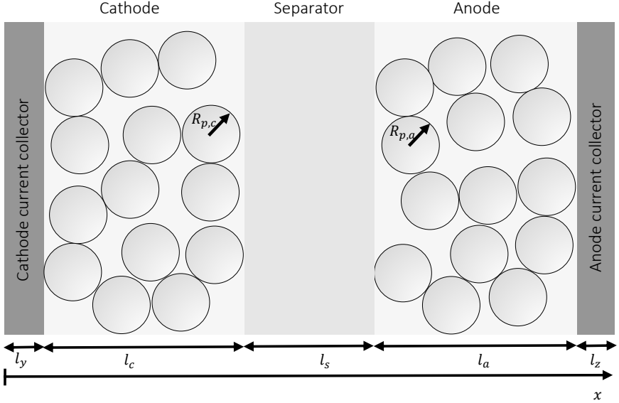
FIGURE 2.1: Schematic of a LIB cell in cross sectional view (figure redrawn based on Ref. [24]). The thickness of the different sections is denoted by l_y for the cathode current collector, l_c for the cathode, l_s for the separator, l_a for the anode, and l_z for the anode current collector. The radius of spherical active material particles is denoted by R_{p,c} for the cathode and R_{p,a} for the anode.
