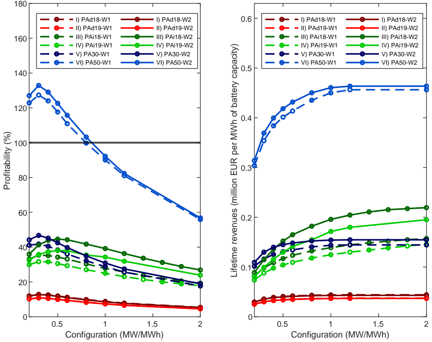
FIGURE 5.8: Profitability (left) and lifetime revenues (right) of battery systems with varying power ratings providing PA services under different electricity market conditions: Day-ahead market in Switzerland from October 2017 to September 2018 ( PAd18 ), day-ahead market in Switzerland in 2019 ( PAd19 ), intraday market in Germany in 2018 ( PAi18 ), intraday market in Germany in 2019 ( PAi19 ), 2030 scenario for Switzerland ( PA30 ), and 2050 scenario for Switzerland ( PA50 ). The model results were obtained for battery systems with the following parameters: Cycle lifetime ( EoL_{cyc} ): 6,000 cycles at 80% DoD, calendar lifetime ( EoL_{cal} ): 15 years, energy efficiency of new battery packs ( \eta^{bat,0} ): 95%. These parameters correspond to the base scenario (#0) in table 5.1. Model results for batteries with Wöhler coefficients W = 1 and W = 2 are shown as dashed and solid lines, respectively. Battery deployment is profitable if the profitability index is higher than 100%, which is indicated by the grey line.
