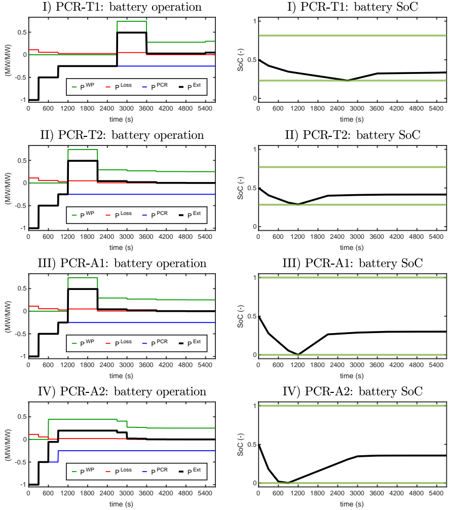
FIGURE 5.19: Provision of PCR under prequalification grid frequencies ( f^P ). The model results were obtained for battery systems with the following parameters: energy capacity ( C_{bat} ): 1 MWh, power rating ( r_{bat} ): 5 MW/MWh, battery state of health ( SoH_{bat} ): 100%, energy efficiency of the battery system ( \eta^{tot} ): 90%, battery state of charge level at t = 0 ( SoC^{init} ): 50%. The left-hand side of the figure shows varying power flows: p^{WP} (green) is the working point, p^{Loss} (red) denotes the internal energy losses in the battery system, p^{PCR} (blue) corresponds to the control signal, and p^{Ext} (black) denotes the total power exchanged between the battery system and the electricity grid. A positive sign for p^{Ext} indicates battery charging, whereas a negative sign indicates battery discharging. All power flows have units [MW/MW], as they are normalized by the amount of PCR capacity provided by the battery system, which is dependent on the electricity market conditions: C^{PCR} = 0.83 \text{ MW} (PCR-T1), C^{PCR} = 1.02 \text{ MW} (PCR-T2), C^{PCR} = 2.40 \text{ MW} (PCR-A1), and C^{PCR} = 3.46 \text{ MW} (PCR-A2). The right-hand side of the figure shows the evolution of the battery SoC level. The green lines indicate the boundaries of the allowed SoC range. In the case studies III and IV, battery operators are allowed to use the full SoC range of the battery system, as no energy reserves need to be kept (i.e., \tau^{Res} = 0 ).
