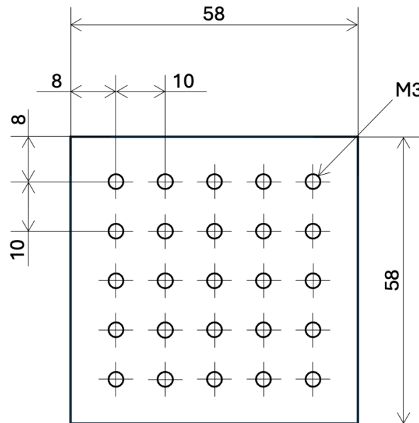
Figure 1 – Dimensions (in mm) and hole pattern of the sample manipulator base plate of I-TOMCAT ES2.
