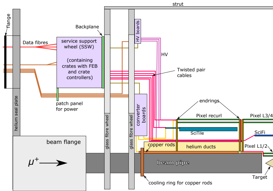
Figure 13.3: Conceptual view of supply system positioning and cable routing ( rz -view, not to scale). All supplies can be disconnected for the extraction of the experiment. The feed-throughs on the helium seal plate are gas-tight.
