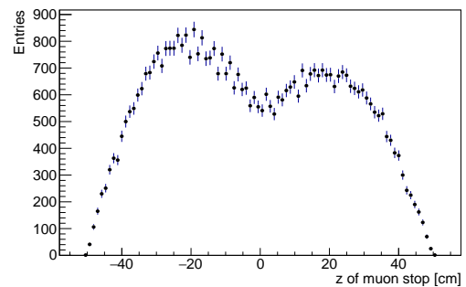
Figure 6.3: Simulated stopping distribution along the beam ( z ) direction for the baseline target.
