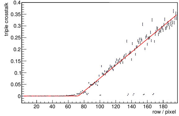
Figure 8.13: Triplet pattern probability due to cross-talk as a function of the row number in MUPiX8. The red solid line shows a fit to the data. For more detail see [68].
