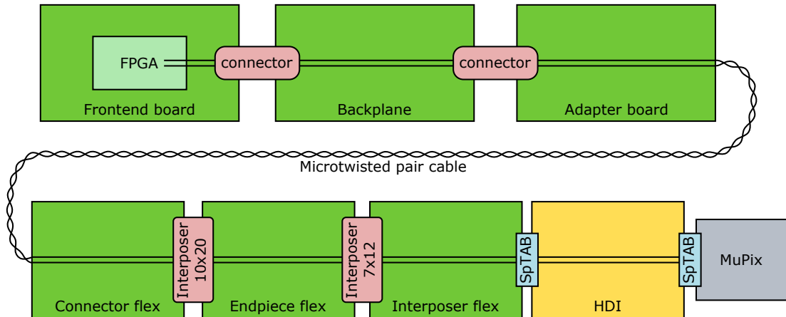
Figure 7.5: Signal path between MuPIX chip and FPGA for a differential readout line. The parts on the top are located on the SSW, the ones on the bottom in the tracker barrels.
