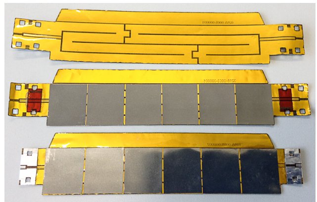
Figure 7.25: Tape heaters for layer 1 and 2. Top to bottom: bare heater with meander, stiffener attached to match final dimensions, dummy chips glued on. Large contact pad pair on both ends used for powering. Chip size 20 \times 23 \text{ mm}^2 .
