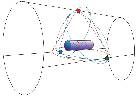
Figure 21.1: Schematic view of a possible alignment system using three cameras. The detector support cage is shown in black, the blue tube represents the detector stations with the endrings shown in red. The three cameras and their fields of view are shown in red, green and blue.
