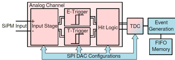
Figure 9.1: Diagram of a MuTRiG channel. After taking signal from SiPM by the input stage, separate signals are provided to the T-Trigger and E-Trigger branches for time and energy discrimination respectively. The discrimination signals are encoded in the hit logic module to generate the combined hit signal, and then converted to digital time stamps after the TDC module. The signal is then buffered in the on-chip memories before being transferred out of the chip. The analogue front-end, TDC and digital modules are configured using a Serial Peripheral Interface (SPI) interface.
