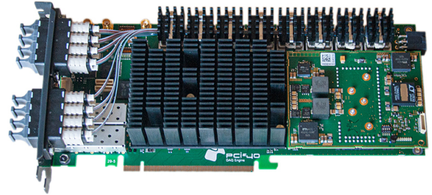
Figure 17.4: PCIe40 board as developed for the LHCb and ALICE upgrades [98,99] and employed as switching board in Mu3e. The large Arria 10 FPGA with two PCIe Gen3 8 lane interfaces is complemented by 48 fast optical receivers and 48 fast optical transmitters.
