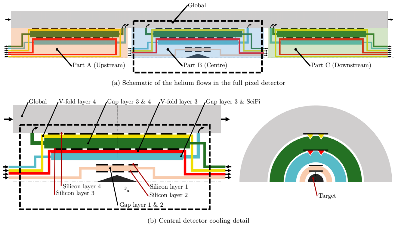
Figure 7.27: Sketch of the helium cooling system for the pixel detector. (a) shows all volumes with its flow directions in a cut view. The system is cylindrically symmetric around the long dashed-dotted line. Some volumes vent into the global flow inside the experiment, indicated by bent arrows. Every circuit is individually controlled for flow and pressure inside the detector volume. (b) shows a cut in the transverse direction as well. The triangles (in red and yellow) indicate the V-fold channels, which exist in pairs for every ladder.
