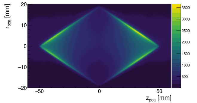
Figure 21.4: Position in r and z of the point of closest approach to the beam line for 3.84 \cdot 10^8 stopped muons; the target is clearly visible. Negative radius is defined to be when the beam line is inside the track circle, positive is outside.
