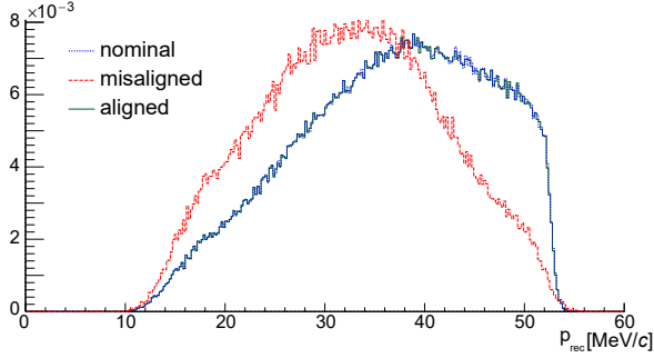
Figure 21.2: Reconstructed momentum of Michel positrons (using only long tracks) for the nominal detector versus the (estimated) detector after assembly and for the aligned detector. Note that nominal and aligned histograms are very similar and thus hard to discern visually.
