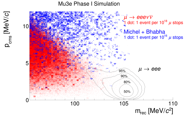
Figure 22.15: Reconstructed invariant mass versus the CMS momentum for signal events, events from radiative decay with internal conversion and accidental background from combinations of Bhabha pairs and Michel electrons. Note that both the internal conversion and Michel and Bhabha simulation use weighted events. The shape of the signal contour at 90% and 95% comes from events where one of the track has an upward fluctuation of the energy loss in the target or the first tracker layers – this leads to a lower reconstructed invariant mass and a larger reconstructed center-of-mass momentum due to the imbalance.
