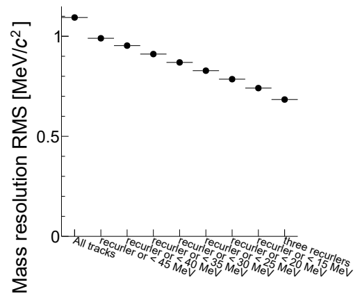
Figure 22.7: Efficiency before timing selection for reconstructing phase-space signal events (top) and the RMS of the corresponding three-particle invariant mass distribution (bottom). Both use the same selection criteria.
