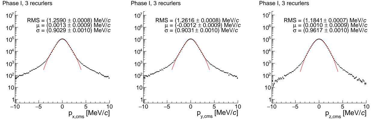
Figure 22.3: Reconstructed decay muon momentum (points) in x , y and z direction (which corresponds to the resolution for p_x , p_y and p_z for muons decaying at rest). Only long tracks enter the analysis. The lines are fits of Gaussian distributions used to estimate the core resolution and to identify biases.
