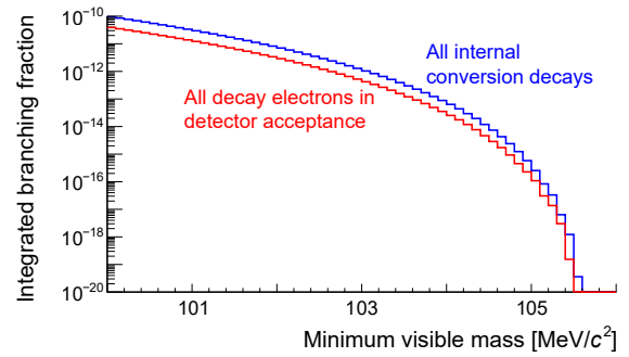
Figure 1.4: Integrated branching fraction of the decay \mu \rightarrow eee\nu\nu for which the invariant mass of the three decay electrons lies above the x axis value. This is shown for all internal conversion decays (blue line) and those with all three decay particles in the detector acceptance, defined as E > 10 MeV and |\cos\theta| < 0.8 (red line). The matrix element was taken from [4].
