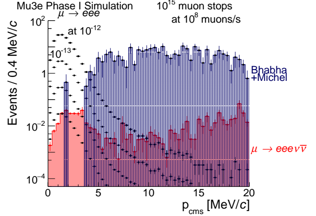
Figure 22.14: Reconstructed center-of-mass system momentum for signal events at various branching fractions ( 10^{-14} and 10^{-15} not labelled) and events from radiative decays with internal conversion. Accidental background from combinations of Bhabha pairs and Michel electrons is also shown. The reconstructed three-particle invariant mass is required to be above 103 \text{ MeV}/c^2 and below 110 \text{ MeV}/c^2 . Note that both the internal conversion and Michel and Bhabha simulation use weighted events.
