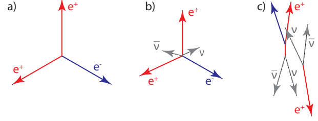
Figure 1.3: Topologies for a) the signal decay, b) the internal conversion decay and c) combinatorial background from two Michel decays with a Bhabha scattering.
