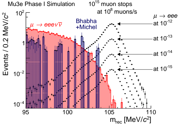
Figure 22.13: Reconstructed invariant mass for signal events at various branching fractions and events from radiative decays with internal conversion. Accidental background from combinations of Bhabha pairs and Michel electrons is also shown. The center-of-mass momentum is required to be less than 4 \text{ MeV}/c . Note that both the internal conversion and Michel and Bhabha simulation use weighted events.
