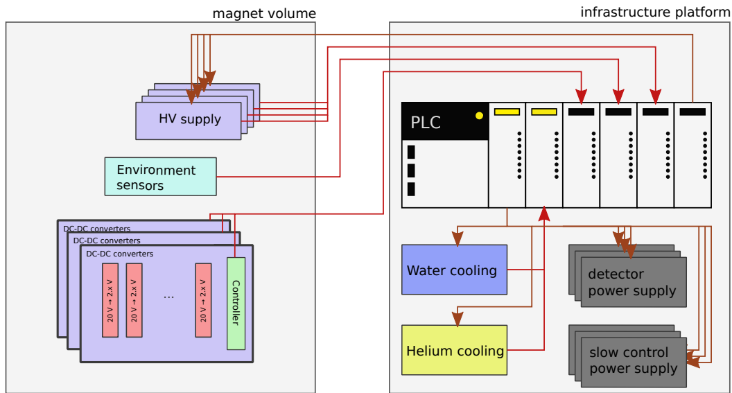
Figure 16.3: Layout of the Mu3e interlock system, directly interconnecting the safety critical sub-systems of the experiment. The PLC is a Siemens SIMATIC S7-series controller.
