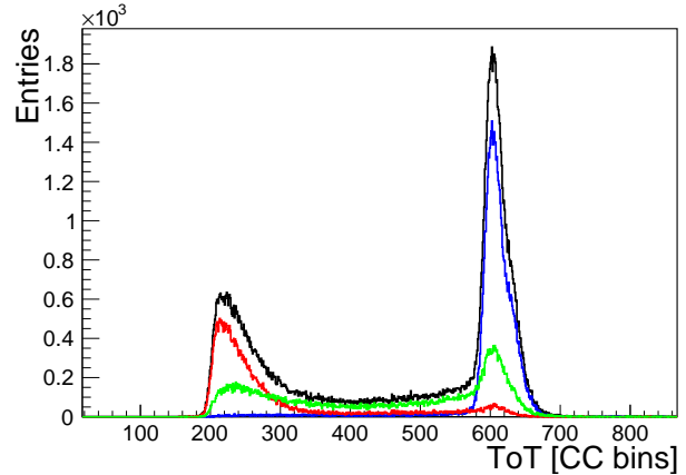
Figure 11.13: Energy deposition in a scintillator tile (black). The spectrum is composed of the Landau peak (blue), a plateau arising from edge effects (particles grazing the tile, green) and a peak from optical cross-talk (red).
