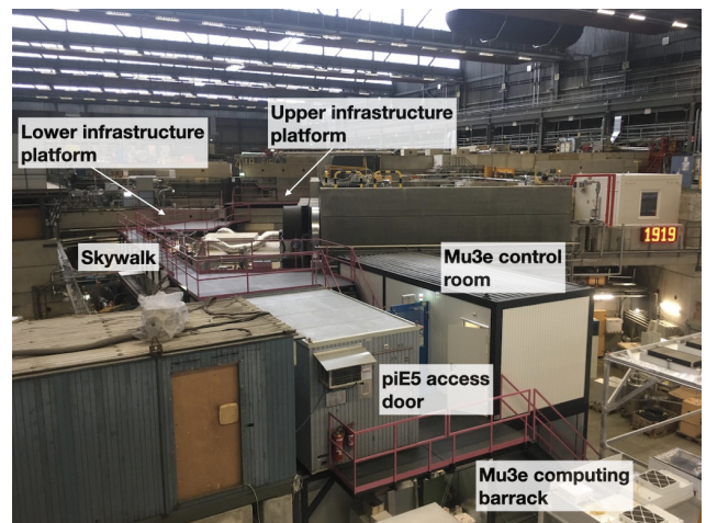
Figure 5.1: The new rear access to the \pi E5 Area with the Skywalk and the two new infrastructure platforms for the Mu3e experiment. In the front, the Mu3e control room and computing barrack are located.
