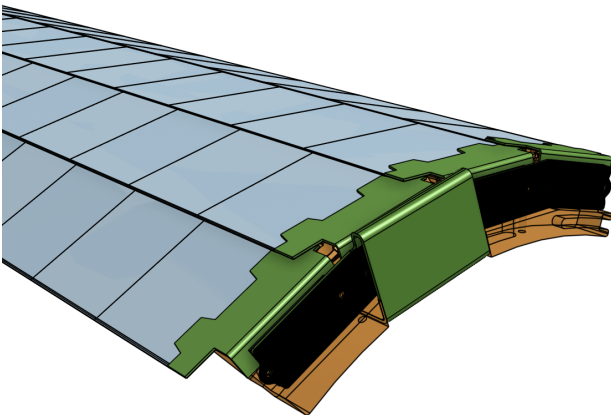
Figure 7.8: Schematic representation of a layer 4 module, integrating four long ladders with 18 MuPIX sensors each. The picture shows one end, including the holding endpiece which also provides the electrical connections. An exploded view can be found in Figure 7.15.
