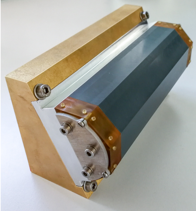
Figure 7.20: Assembly tool for layer 2 modules. Tilting of the full tool and sliding of the grey block allows to bring every facet into the horizontal position.
