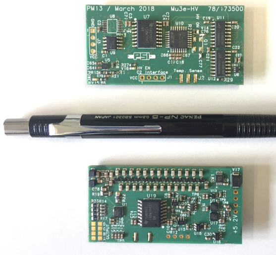
Figure 14.4: Prototype of the high-voltage generator board with top side (upper picture) and bottom side (lower picture).
