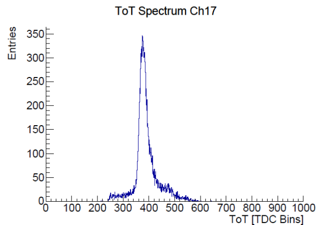
Figure 9.8: The time-over-threshold (ToT) of minimum-ionising electrons recorded on channel 17.
