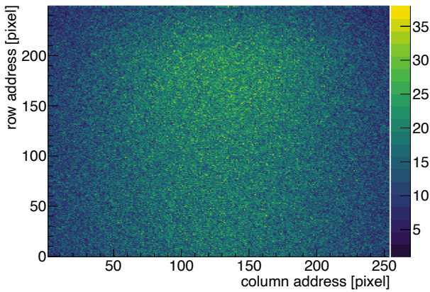
Figure 8.20: MUPiX10 hit map in a beam of 3 GeV/c electrons measured at DESY. The active area is 4.1 cm 2 .
