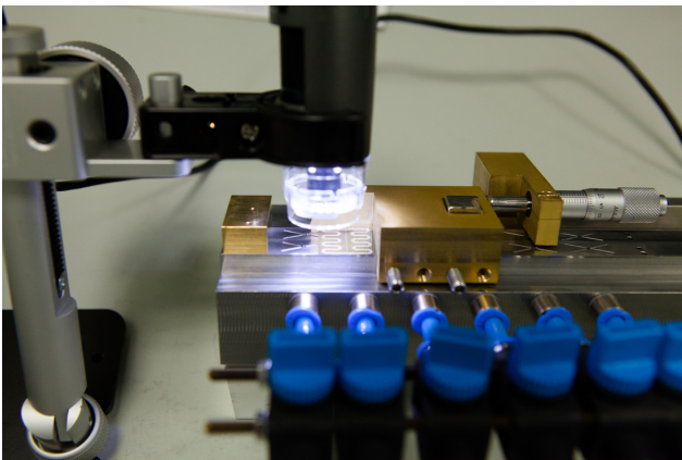
Figure 7.18: Assembly tool for the inner tracking ladders. Brass sliding block in the middle is guiding a prototype chip into position. Brass stop edge to the left. Micrometer screw to the right. Microscope to monitor position at the top.
