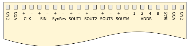
Figure 7.12: Conceptual MuPIX pad layout on the HDI. Depending on location, either SOUT1 to SOUT3 or SOUTM is connected to accommodate for different data rate needs (vertex or recur layers, respectively). Power and ground have multiple pads to reduce effects of voltage drop.
