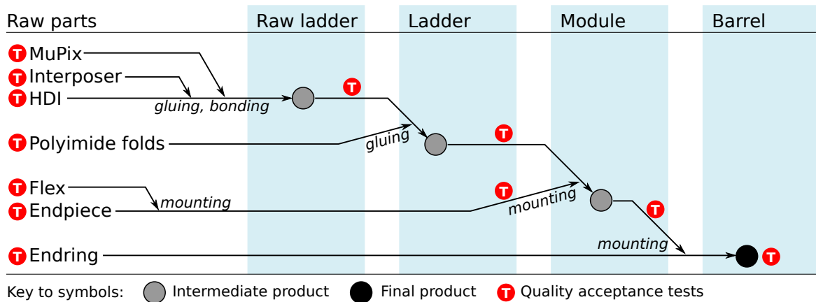
Figure 7.17: Module manufacturing workflow and quality points. Only main steps are shown.
