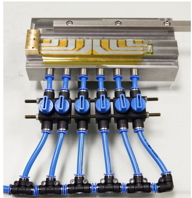
Figure 7.19: Prototype ladder for the inner pixel layers after gluing on mounting tool.
