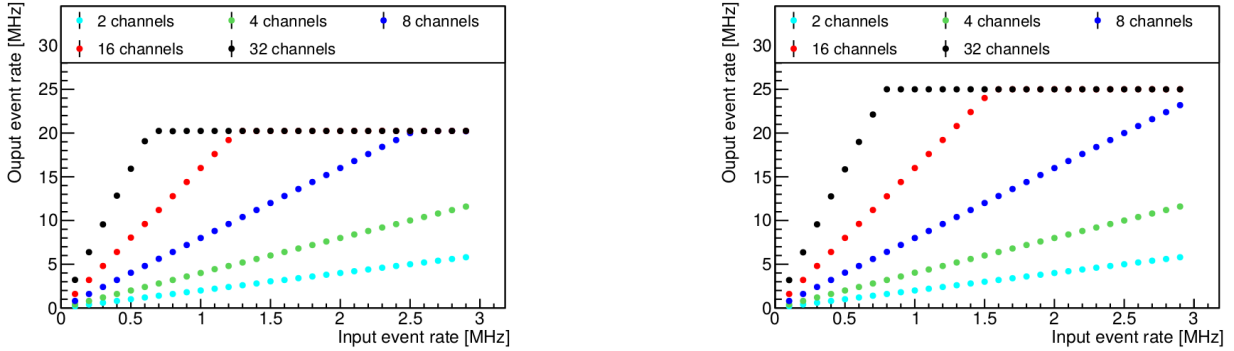
Figure 9.5: Event rate measurements for the standard output event structure (left) and short output event structure (right).
