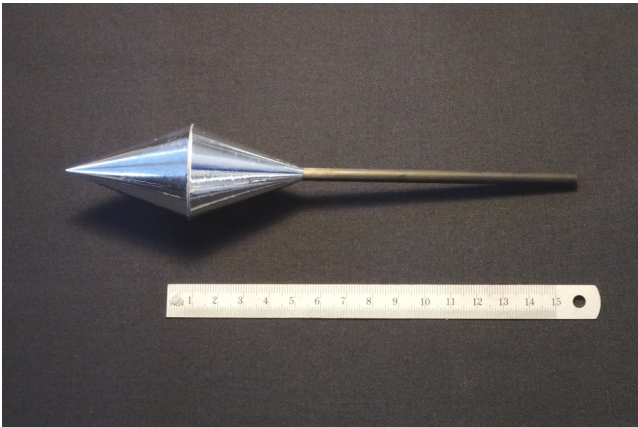
Figure 6.5: Hollow double-cone muon stopping target made of aluminised Mylar foil.
