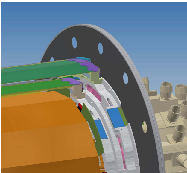
Figure 7.16: Endring situation shown with modules inserted in layers 3 and 4.
