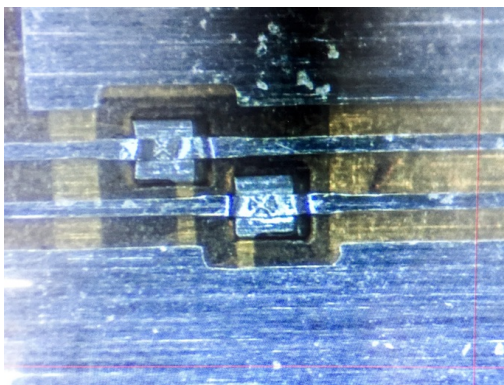
Figure 7.10: Photograph of two SpTA-bonds on a test flex-print produced by LTU Ltd [25].
