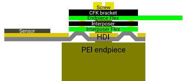
Figure 7.7: Schematic representation of the connections within an interposer at the end of an HDI flex.
