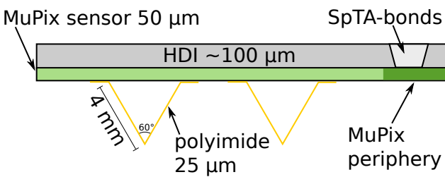
Figure 7.9: Cross section of an outer layer ladder. From top to bottom: HDI, MuPIX sensor, polyimide support structure. Not to scale.
