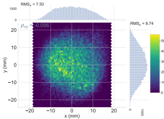
Figure 3.10: Estimated beam profile at the Mu3e target position.
