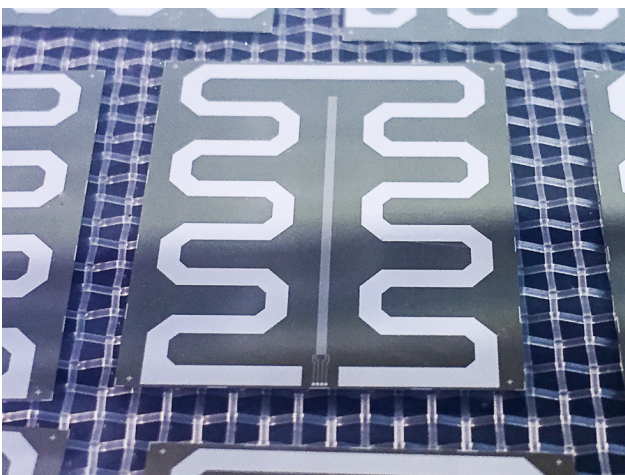
Figure 7.23: Silicon heater chip. The large meander for heating the chip and a narrow meander used as an RTD can both be seen. Contact pads are arranged on the bottom edge corresponding to the final chip connection locations.
