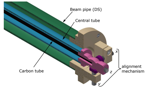
Figure 6.6: Cross section of alignment mechanism. The setup is spring-loaded towards the two screws and allows an adjustment of the target position in 3 coordinates. The direction of the spring is in the bisecting line with respect to the two screws and is in this view therefore hidden by the holder.
