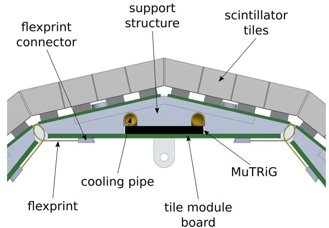
Figure 11.6: Tile detector with readout electronics. The tile module is divided into a PCB hosting the MuTRiG chips and 2 \times 13 PCBs hosting the SiPMs. The SiPM boards are connected to the MuTRiG board via flex cables. The tile readout board is placed on the cooling structure, connecting the tile sub-modules to the front-end FPGA readout board.
