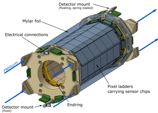
Figure 7.6: Schematic view of the vertex pixel barrel. Each of the 8+10 ladders carry 6 sensor chips. Endrings (split in halves) provide the mechanical support to the ladders.
