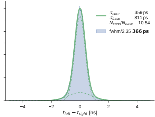
Figure 10.15: Time resolution of a 4 layer SCSF-78MJ SciFi ribbon extracted from clusters with at least 2 active columns. No channel by channel time offset correction has been applied.
