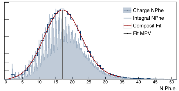
Figure 10.13: Light yield of a cluster (see text) for a m.i.p. crossing a three-layer SCSF-78MJ fibre ribbon prepared with clear epoxy. The integral NPhe is obtained by integrating the charge in a region of \pm 0.5 ph.e. around each peak (integer). A convolution of a Gaussian and of a Landau is used to fit the data and the MPV of the spectrum is marked with the vertical line.
