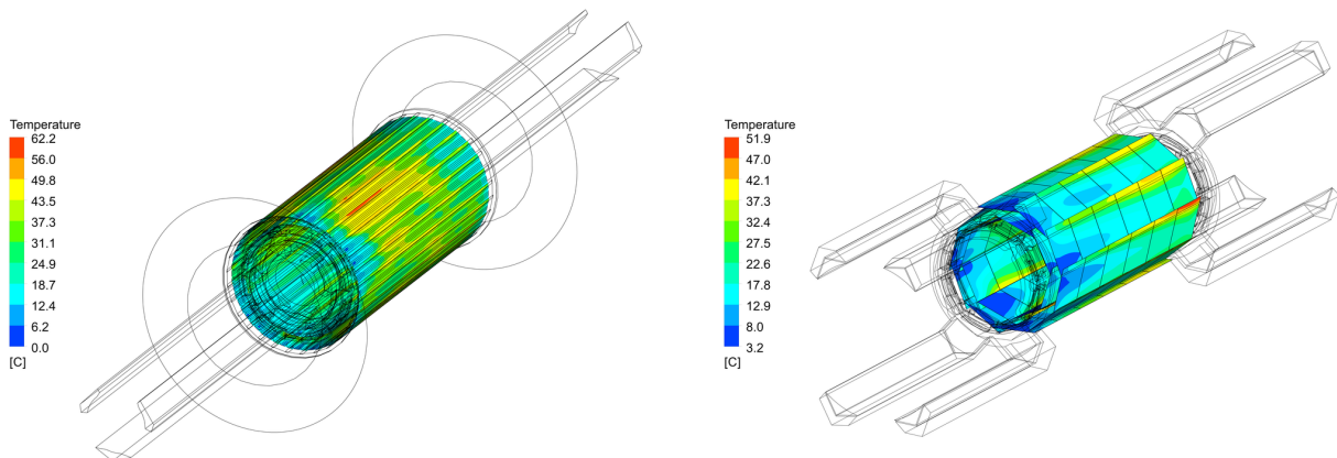
Figure 7.28: Simulated \Delta T distribution of the silicon in the tracking detector for a power dissipation of 400 \text{ mW/cm}^2 (non-uniform distribution, more heat power at periphery edge). Inlet gas temperature is T = 0^\circ\text{C} Left: full barrel. Right: vertex barrel inside the full barrel.
