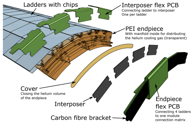
Figure 7.15: Exploded view of the outer layer module assembly. The end piece region provides a manifold for distributing the helium cooling gas and holds the flexible circuits to connect ladders to a single electrical connection matrix on the bottom.
