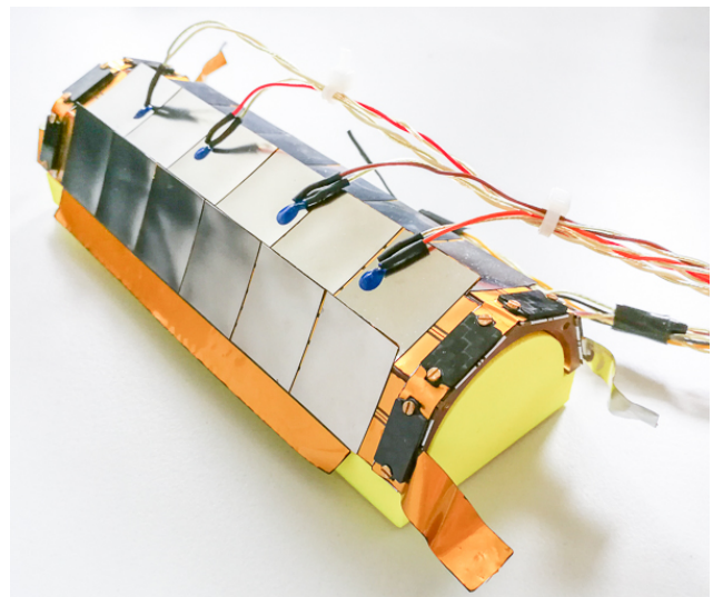
Figure 7.26: Layer 1 half shell made with tape heaters and stainless steel dummy chips, placed on a handling block (yellow). RTDs attached with conductive glue for temperature profiling in cooling tests.
