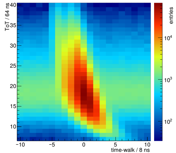
Figure 8.15: Correlation between ToT and time-walk (ToA minus scintillator reference after correcting for individual pixel delays) for MUPIX8 using a 4 GeV electron beam at DESY. Plot from [63].
