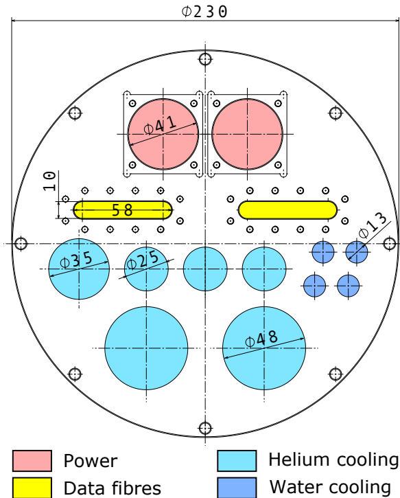
Figure 13.4: Drawing of the cabling flange. Additional ports will be added for auxiliary use. Dimensions in mm.
