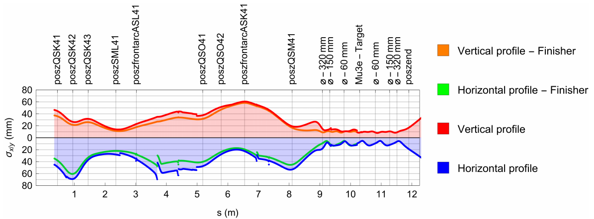
Figure 3.9: Horizontal and vertical beam envelopes for ‘all’ particles started in the simulation or only for those that reach the centre of the solenoid (‘finishers’). Due to the losses along the beamline on apertures and other restrictions the two envelopes converge at the center of the Mu3e target.
