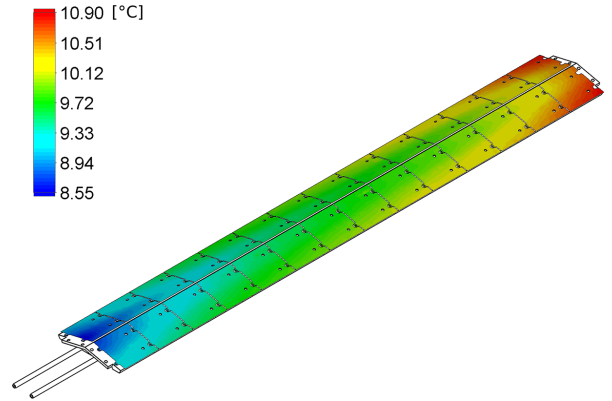
Figure 11.17: Simulated temperature of the SiPM PCBs. The temperature of the cooling water was set to 1 °C at a flow speed of 1 m/s, while the environment temperature was set to 50 °C.
