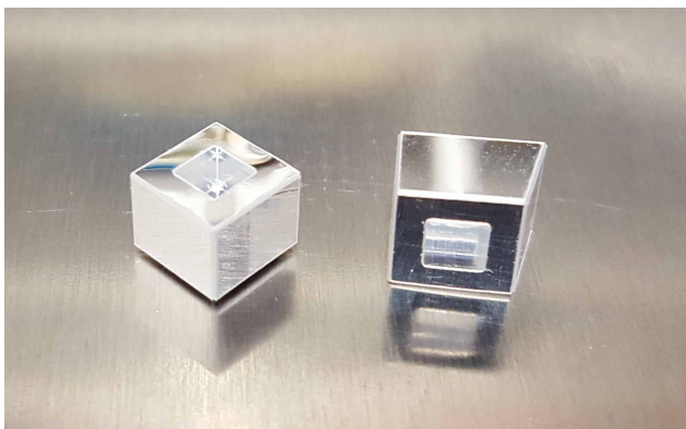
Figure 11.4: Individual tiles wrapped with ESR reflective foil.
