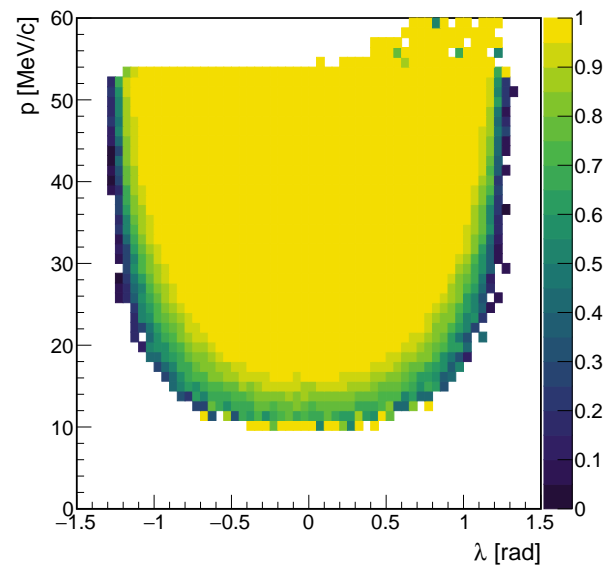
Figure 19.1: Ratio of reconstructed short tracks to generated particles producing a hit in each of the four detector layers as a function of momentum p and inclination angle \lambda (see section 2.2 for a definition of the coordinate system). The entries at high momentum in the forward direction ( \lambda > 0 ) are from decays in flight.
