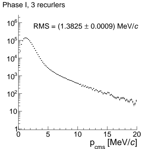
Figure 22.4: Magnitude of the center of mass system momentum reconstructed for signal events with three recurlers required.
