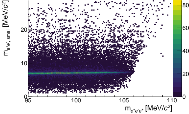
Figure 22.12: Small invariant mass of e^+e^- pairs versus e^+e^-e^+ invariant mass for accidental combinations of a Bhabha e^+e^- pair with a Michel positron. Simulated kinematics weighted with the track reconstruction efficiency.
