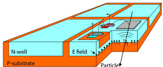
Figure 8.1: Sketch of the HV-MAPS detector design from [23].
