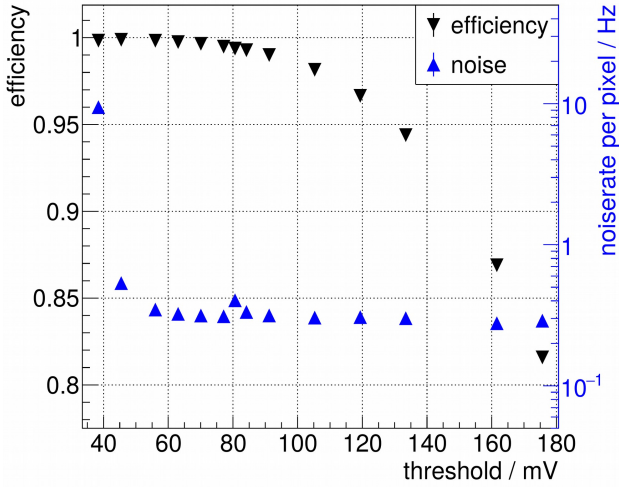
Figure 8.11: Hit efficiency and noise as a function of the charge threshold for the MUPiX8 sensor 084-2-03 (80 \Omega cm, thickness 62 \mu m) as measured for 4 GeV electrons for a beam inclination angle of 0°. The bias voltage was set to -60 V and the pixel cells were untuned. Plot from [68].
