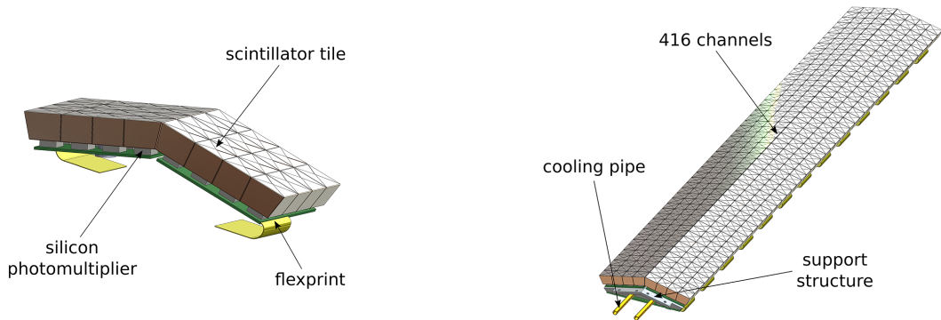
(a) The tile detector base unit consisting of 32 scintillator and SiPM channels. The sensors are mounted on a flex-rigid PCB. CAD rendering.
