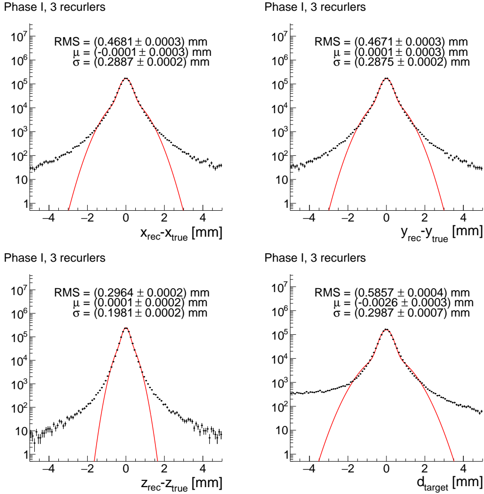
Figure 22.1: Vertex resolution for simulated signal decays (points). Three tracks with recurlers are selected. The fits (lines) are the sum of two Gaussian distributions and the quoted \sigma is the area-weighted mean. Top left in x , top right in y , bottom left in z and bottom right in the distance to the target; negative target distances denote a reconstructed vertex position inside the target.
