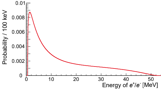
Figure 1.5: Energy spectrum of all electrons and positrons from internal conversion decays.
