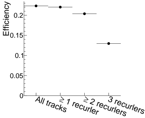
Figure 22.6: Total efficiency for reconstructing phase-space signal events as a function of the required number of recurling tracks. This includes the geometrical detector acceptance, track and vertex reconstruction and selection inefficiencies.
