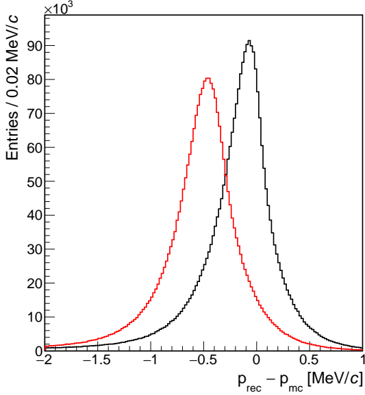
Figure 19.5: Difference between reconstructed and generated momentum after the first detector layer, for long tracks with (black) and without (red) energy loss correction. The average momentum resolution is about 0.2 MeV/c, the correction it improves by 10%.
