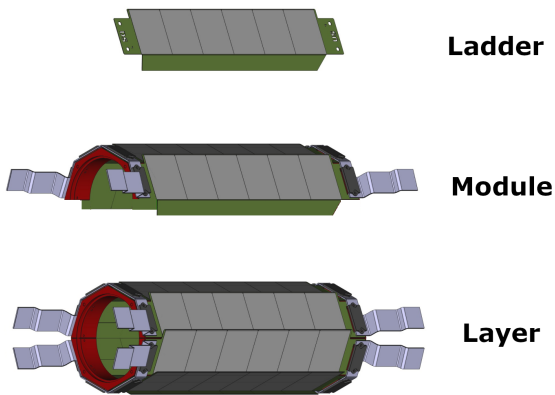
Figure 7.3: 3D-model reproduction of the Tracker Layer 1 assembly, from single ladder to module to full layer.
