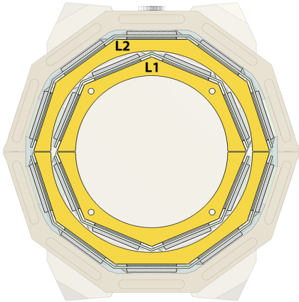
Figure 7.14: Holding endpieces and endrings of the inner layers with the octagonal (layer 1) and decagonal (layer 2) geometry, shown in yellow.
