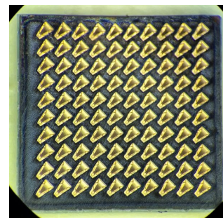
Figure 7.13: Interposer ZA8 from Samtec, version with 10 × 10 connections. The pins have a pitch of 0.8 mm
