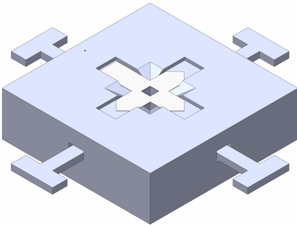
Figure 11.8: Sketch of the tile wrapping tool with a foil on top.
