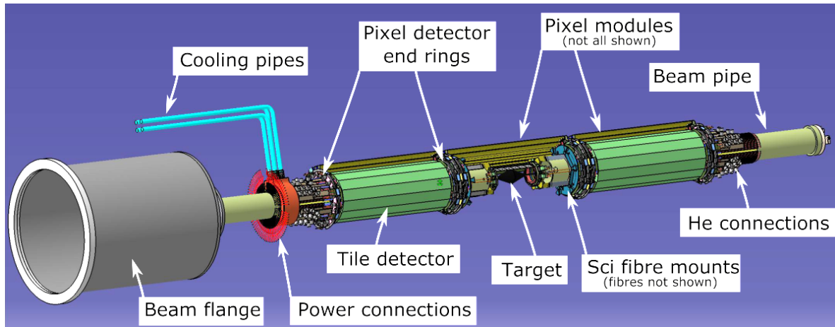
Figure 13.2: The Mu3e experiment mounted on the beam pipes. Not shown are the detector cage and supplies. Some parts have been partially removed for visibility.
