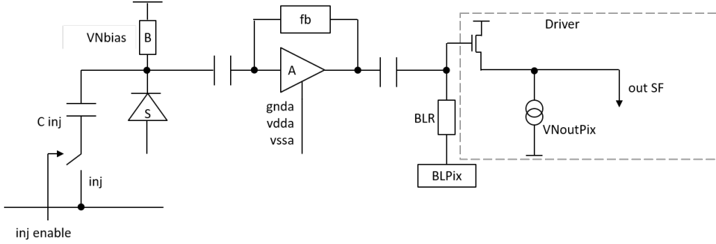
Figure 8.7: Schematic of the pixel cell analogue electronics in the MUPIX chips. The main components are from left to right: charge injection (C Inj), the charge collecting diode (S), the n-well bias restoration circuit (B), the amplifier (A) with the feedback line (fb), the baseline circuit with base line restoration (BLR) and the source follower (out SF). See text for further detail.
