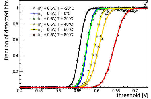
Figure 8.17: MUPix7 response to a constant injected charge as a function of the comparator threshold (“s-curve”) for different temperatures ranging from -20 to +80^\circ\text{C} [72]. Note that due to the 2-stage amplifier in MUPix7 high voltages correspond to low signals (thresholds). For this measurement the baseline is at about 0.8 V.
