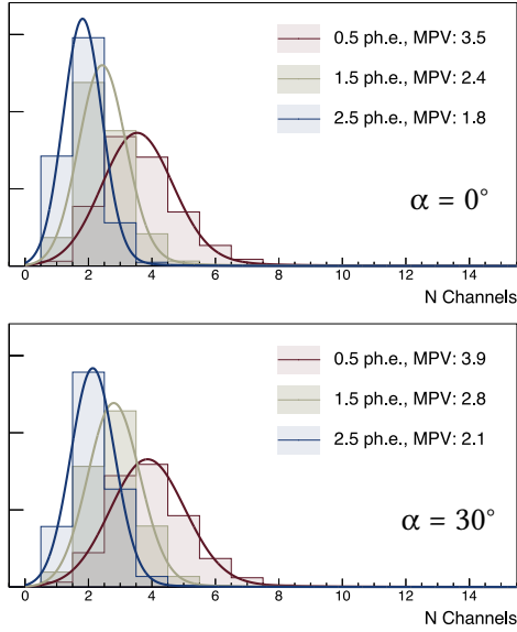
Figure 10.14: Cluster size for a particle crossing the ribbon at two different angles and different thresholds. Electrons from a radioactive ^{90}\text{Sr} source are used for this measurement. An angle of \alpha = 0^\circ describes a perpendicular crossing.
