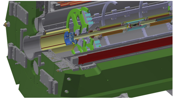
Figure 5.5: Connection of the Mu3e detector to the muon beam line is achieved through a custom bellows assembly inside the solenoid.
