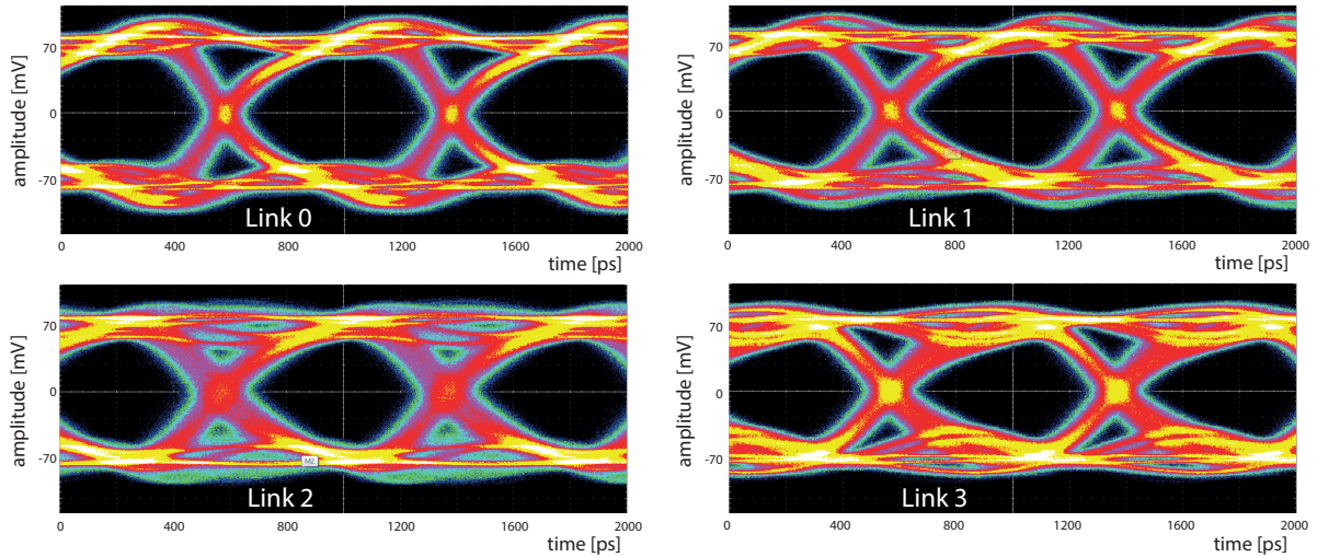
Figure 8.18: MuPIX8 serial data outputs at 1.25 Gbit/s. The links 0, 1, and 2 refer to the pixel matrices A, B and C. Link 3 is switchable. Plot modified from [73].
