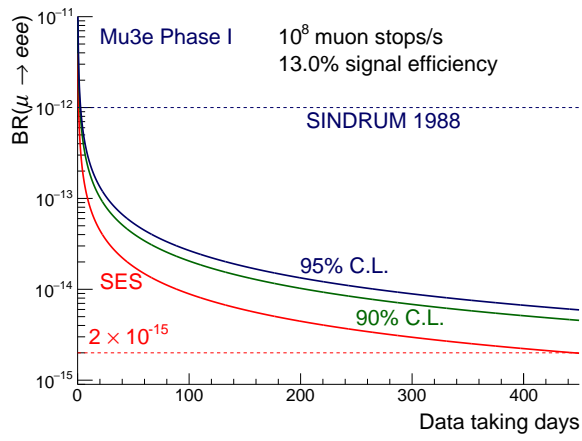
Figure 22.16: Single event sensitivity (SES) and the corresponding 90% and 95% C.L. upper limits versus data taking days for the phase I Mu3e detector.
