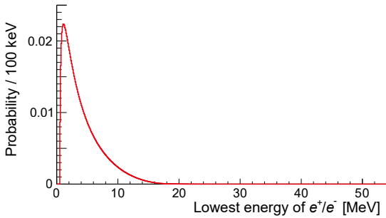
Figure 1.6: Energy spectrum of the electron or positron with lowest energy from internal conversion decays.
