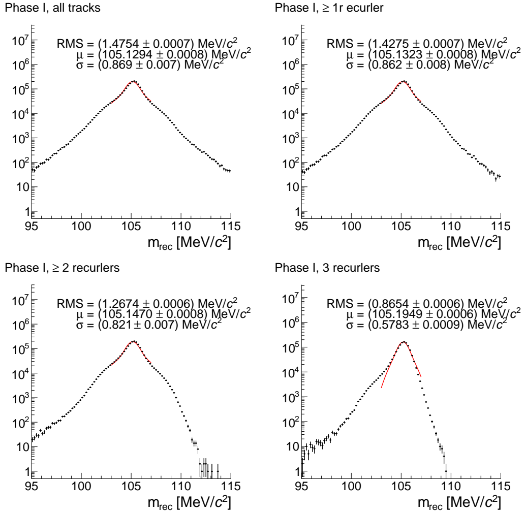
Figure 22.5: Reconstructed muon mass m_{rec} for signal decays for all tracks (top left), at least one recurler (top right), at least two recurlers (bottom left) and three recurlers (bottom right). The fits are the sum of two Gaussian distributions and the quoted \sigma is the area-weighted mean; the main purpose of the fit is to guide the eye and highlight the non-symmetric resolution distribution.
