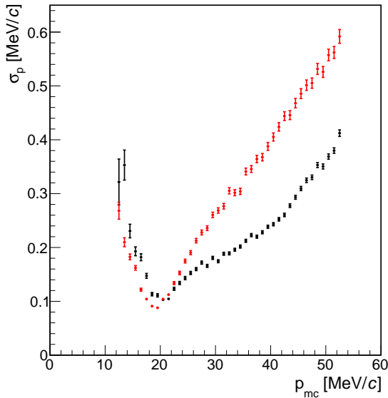
Figure 19.3: Momentum resolution \sigma_p as a function of the generated total momentum p_{mc} for 6-hit (black) and 8-hit (red) long tracks. The momentum resolution has a minimum for tracks that traverse half a circle outside the outermost pixel layer.
