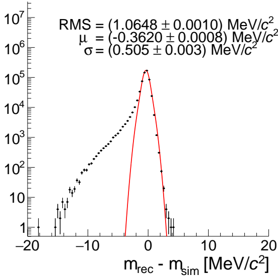
Figure 22.8: Resolution of the mass reconstruction for internal conversion events with a visible mass above 90 \text{ MeV}/c^2 for three recurling tracks and a CMS momentum of the three particle system of less than 8 \text{ MeV} .
