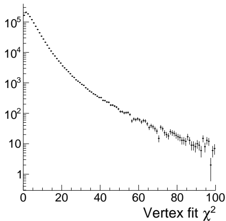
Figure 22.2: \chi^2 of the the vertex fit for signal events. The number of degrees of freedom is three [134], note however that the finite resolution of the pixel detector is ignored in the current implementation of the vertex fit and the distribution is thus not expected to follow a \chi^2 distribution with three degrees of freedom.
