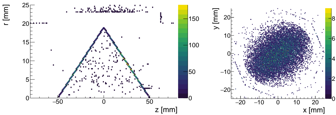
Figure 22.10: Longitudinal view (left) and transverse view (right) of muon decay vertices leading to a positron that then interacts via Bhabha scattering in the target resulting in an electron and a positron both in the detector acceptance in the target region for 1.9 s of running at 1 \cdot 10^8 muon stops per second. The distribution corresponds to the muon stopping distribution in the target region, showing no unexpected source of positrons.
