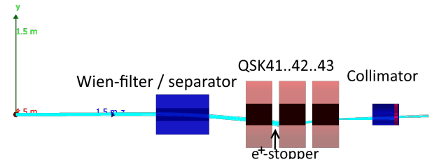
Figure 3.6: Demonstration of beam positron contamination vertically separated post Wien-filter being swept-back into the acceptance at the collimator by QSK42/43.
