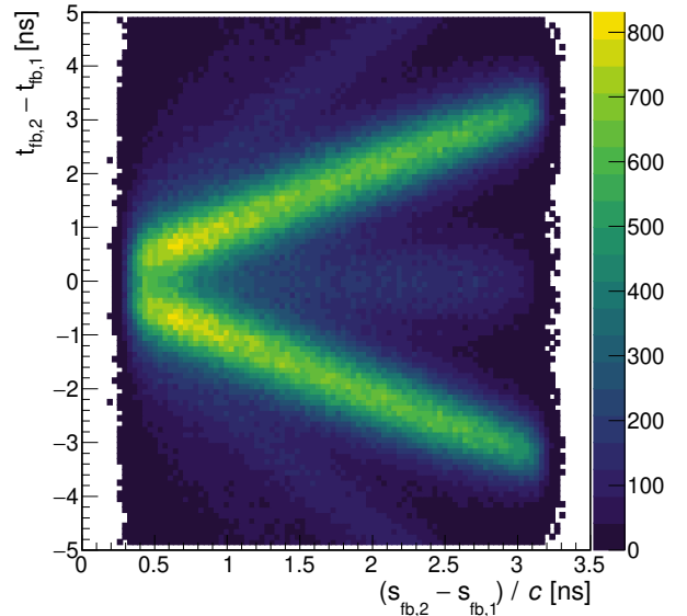
Figure 19.6: Time difference between fibre clusters assigned to 8-hit long tracks as a function of distance along the trajectory. The upper branch corresponds to the correct charge assignment and direction of rotation, and the lower branch to the wrong charge assignment.
