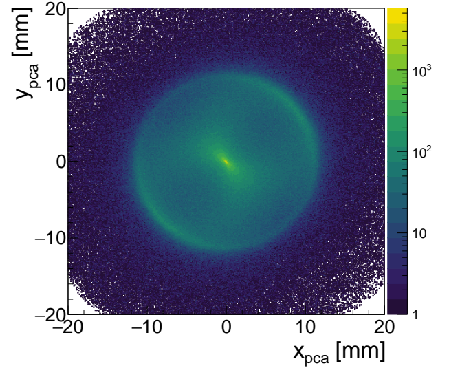
Figure 21.3: Position in x and y of the point of closest approach to the beam line for a 1 mm slice in z at -20 mm for 3.84 \cdot 10^8 stopped muons. The target is clearly visible at its nominal position. The accumulation of entries towards the origin is a feature of the reconstruction method.
