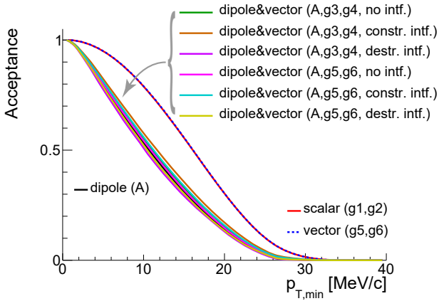
Figure 1.2: The acceptance, defined as the fraction of \mu \rightarrow eee decays in which all decay products have transverse momenta above p_{T,min} , against p_{T,min} for different effective LFV models. The black line corresponds to pure dipole and the red and blue dotted lines (on top of each other) to pure four-fermion contact interaction models (no penguin contribution); the other lines correspond to a mixture of dipole and vector interactions. Based on [3].
