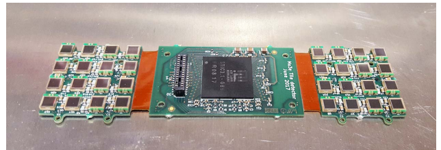
Figure 11.10: Tile matrix board assembled with SiPMs and a BGA packaged STiC 3.1 ASIC.
