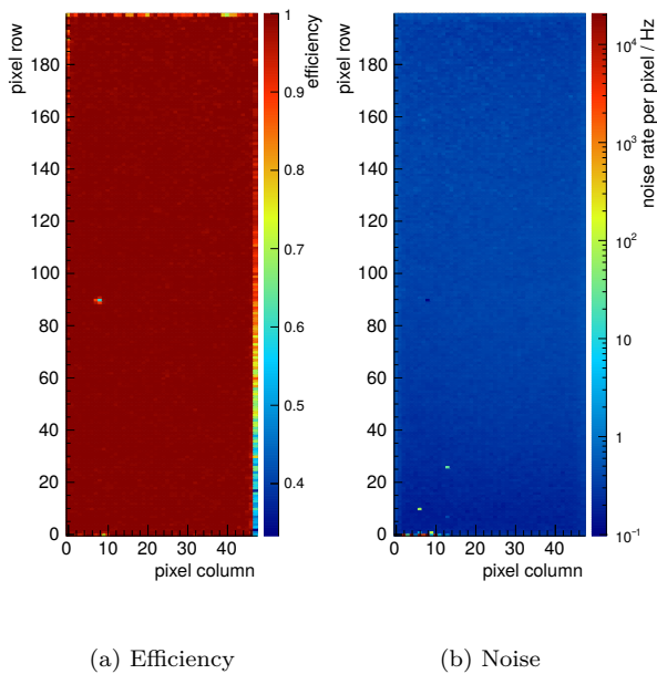
Figure 8.10: Efficiency and noise maps for the MuPIX 8 sensor 084-2-03 (80 \Omega cm) at a threshold of 56 mV and a bias voltage of -60 V. Note that the noise was measured during beam and that the noise rate also includes non-reconstructed beam particles. Plot from [68].
