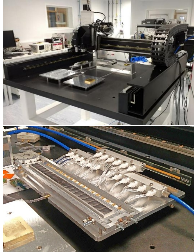
Figure 7.21: Robotic gantry (upper figure) for placement of 17 or 18 MuPIX chips on the vacuum jig (lower figure).
