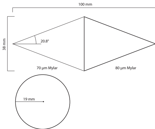
Figure 6.1: Dimensions of the baseline design target. The muon beam enters from the left. Note that the material thickness is not to scale.
