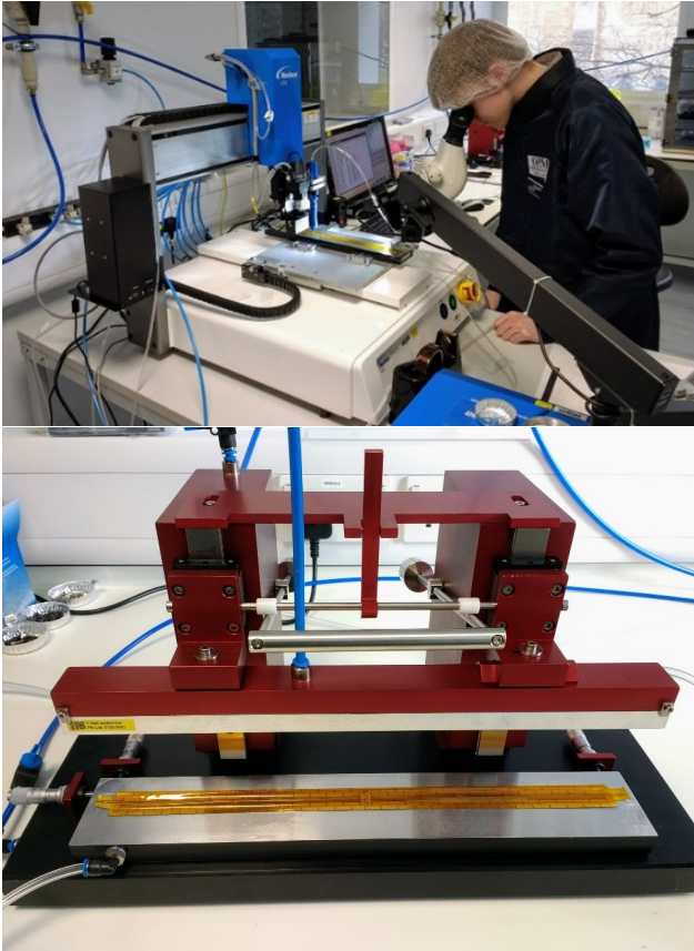
Figure 7.22: Glue dispensing robot (upper figure) and custom tooling for the gluing of v-channel reinforcements (lower figure).
