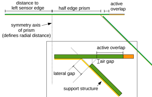
Figure 7.4: Design of the MuPIX ladder overlap region of pixel layer 1. The green region indicates the active part of the sensor, the orange part the inactive periphery and the yellow part the polyimide support structure. The lower edge shows a zoom into the overlap region. Note that the sensor thicknesses are not to scale.
