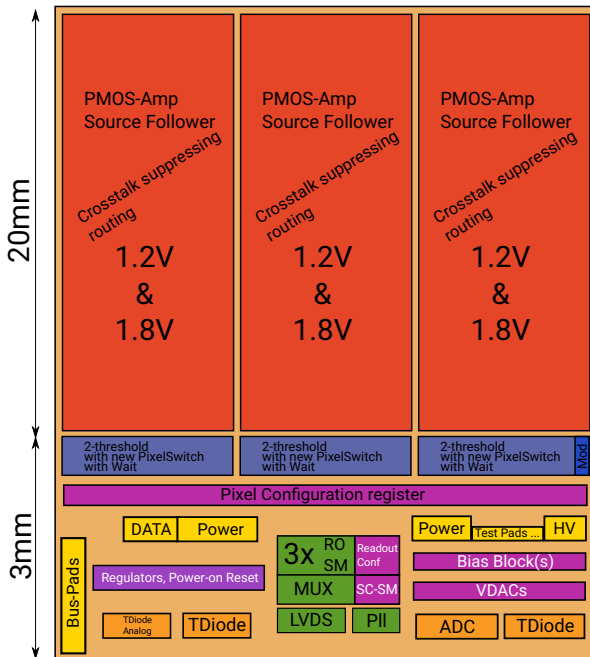
Figure 8.5: MuPix10 block diagram (not to scale).
