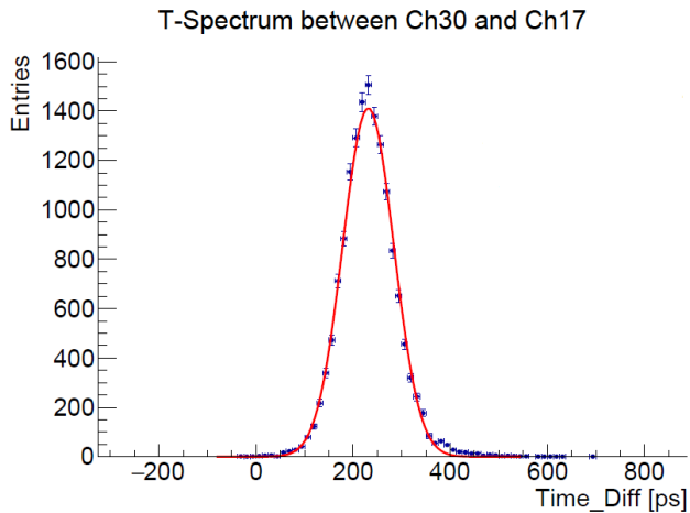
Figure 9.9: Coincidence timing spectrum between channel 30 and 17.
